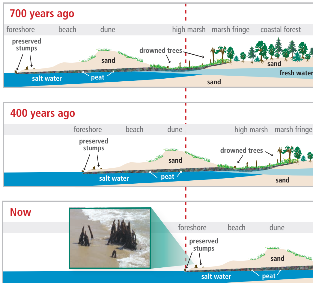
Figure 2. Series of images explaining marine transgression.
