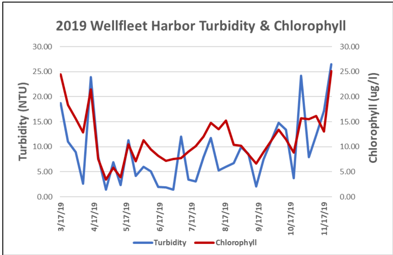
Weekly mean turbidity and chlorophyll as measured in Wellfleet Harbor during 2019.
