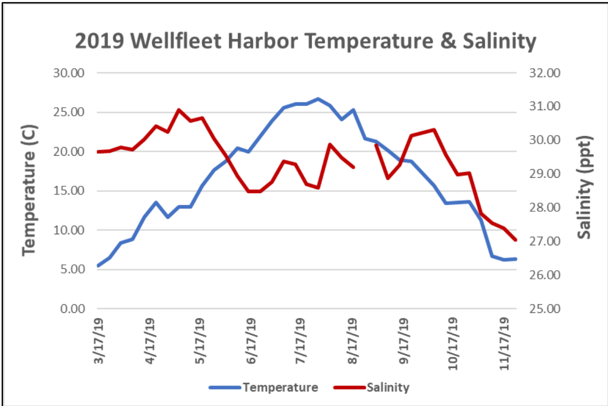
Weekly mean water temperature and salinity as measured in Wellfleet Harbor during 2019.
