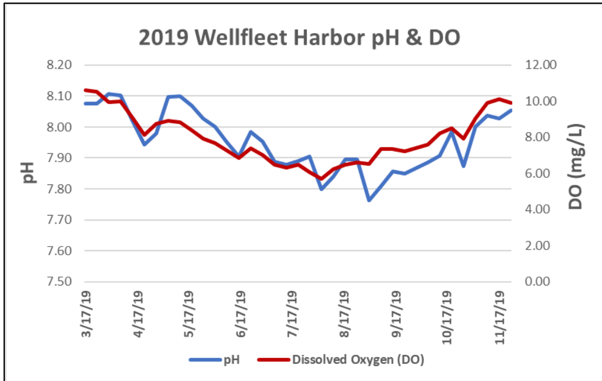
Weekly mean pH and dissolved oxygen as measured in Wellfleet Harbor during 2019.
