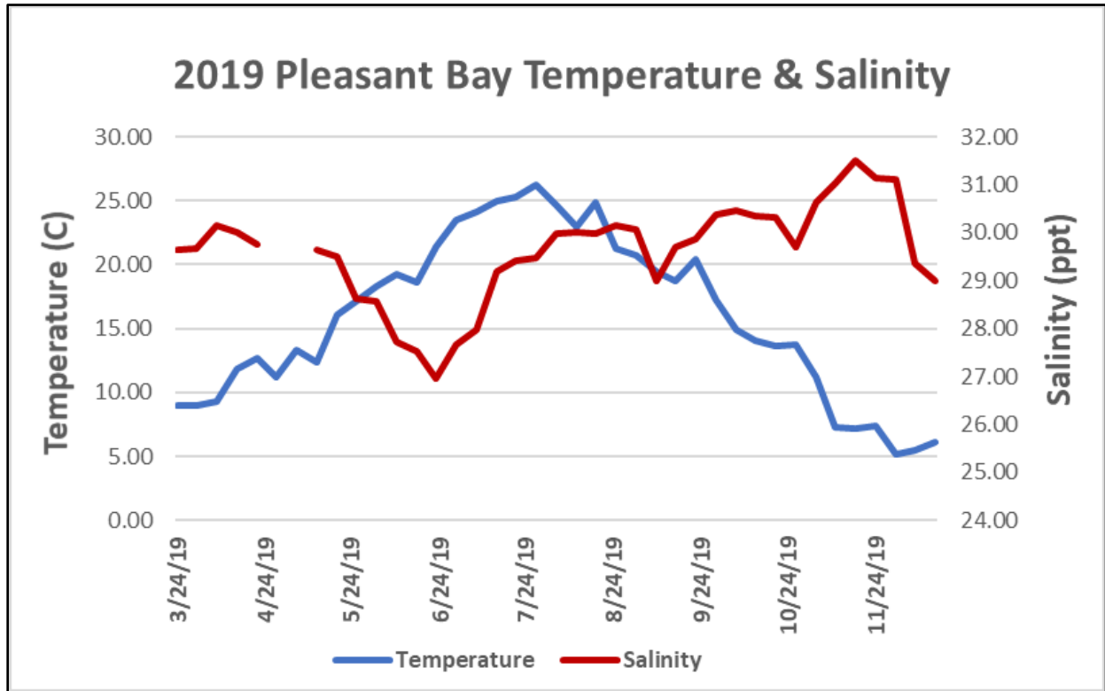
Weekly mean water temperature and salinity as measured at Portanimicut Landing in Pleasant Bay during 2019.
