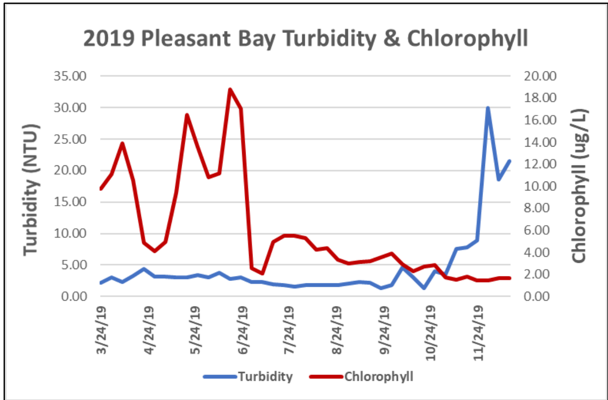
Weekly mean turbidity and chlorophyll as measured at Portanimicut Landing in Pleasant Bay during 2019.
