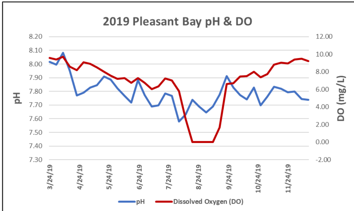
Weekly mean pH and dissolved oxygen as measured at Portanimicut Landing in Pleasant Bay during 2019.
