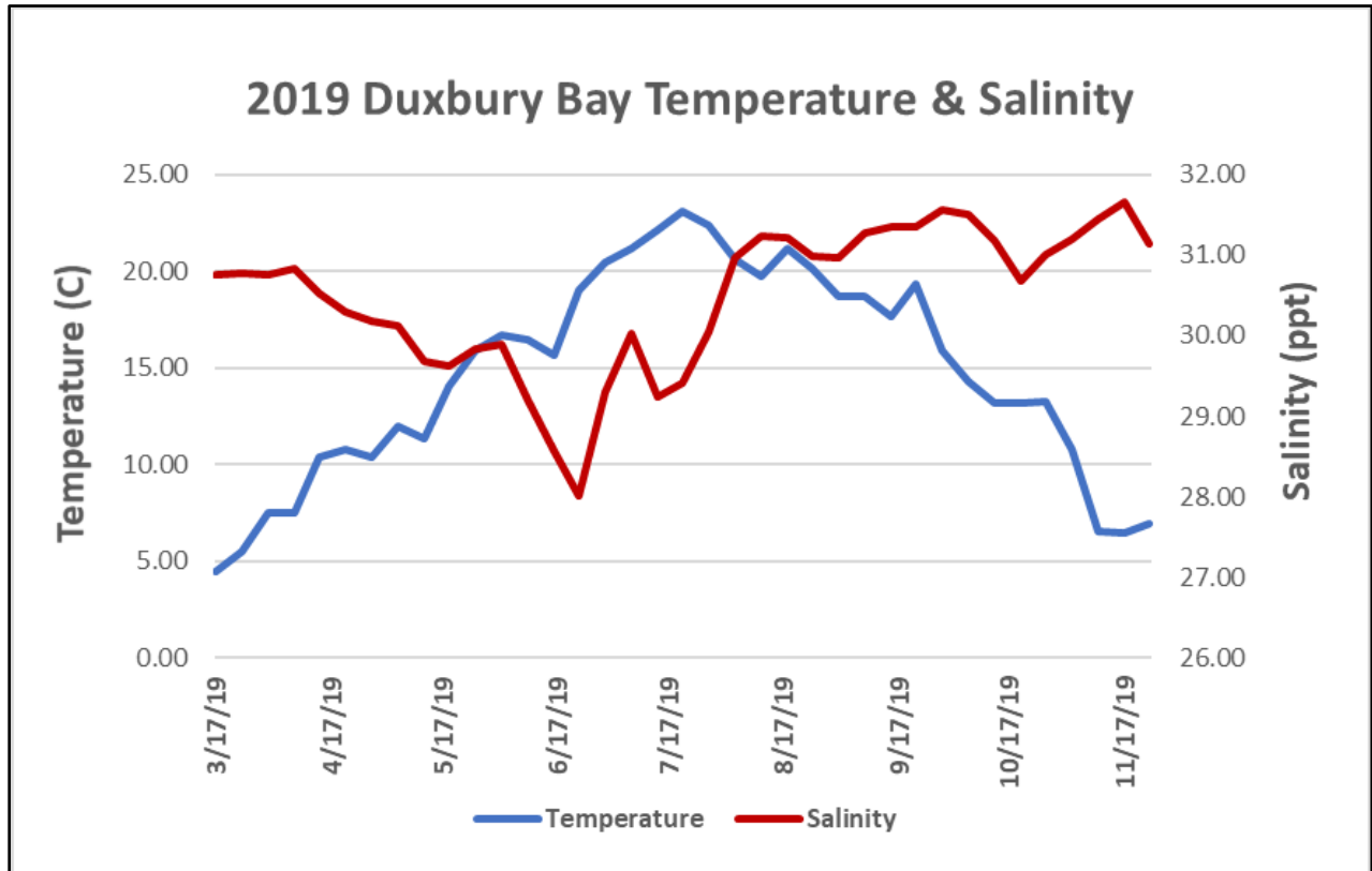
Weekly mean water temperature and salinity as measured in Duxbury Bay during 2019.
