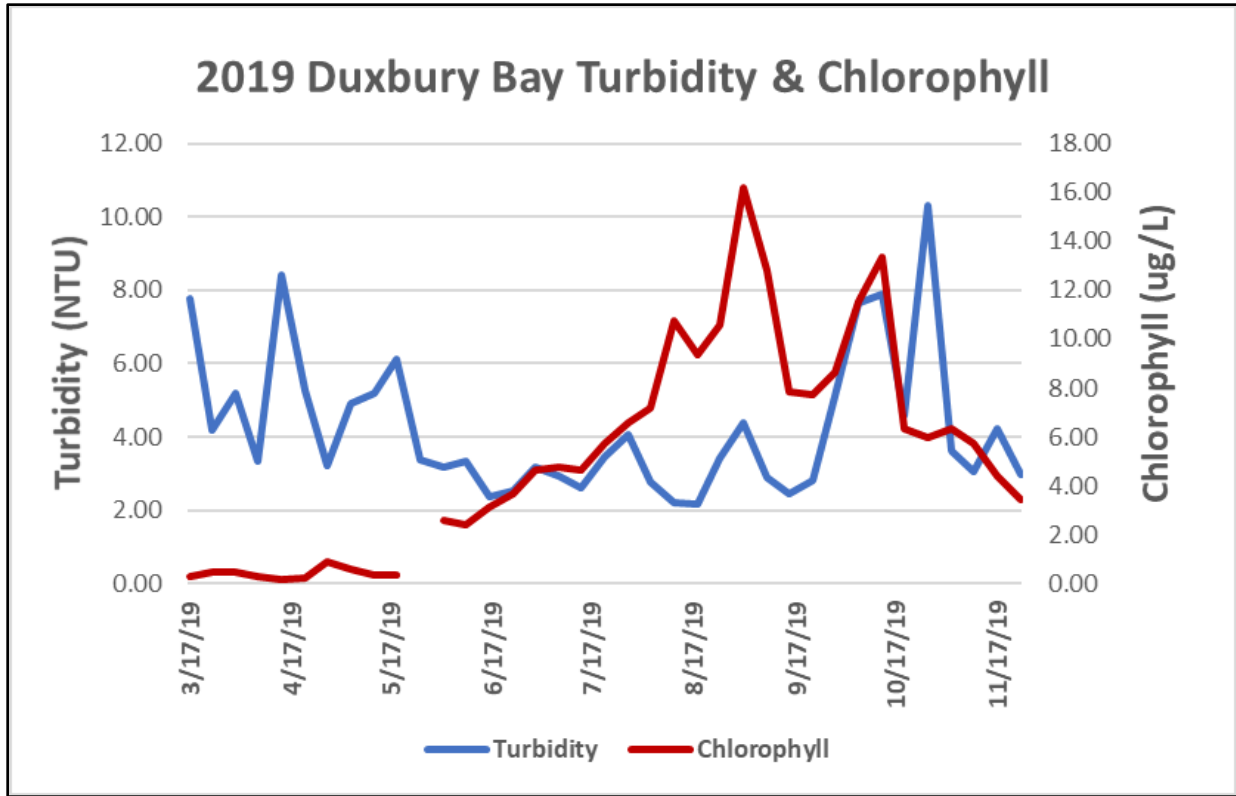
Weekly mean turbidity and chlorophyll as measured in Duxbury Bay during 2019.
