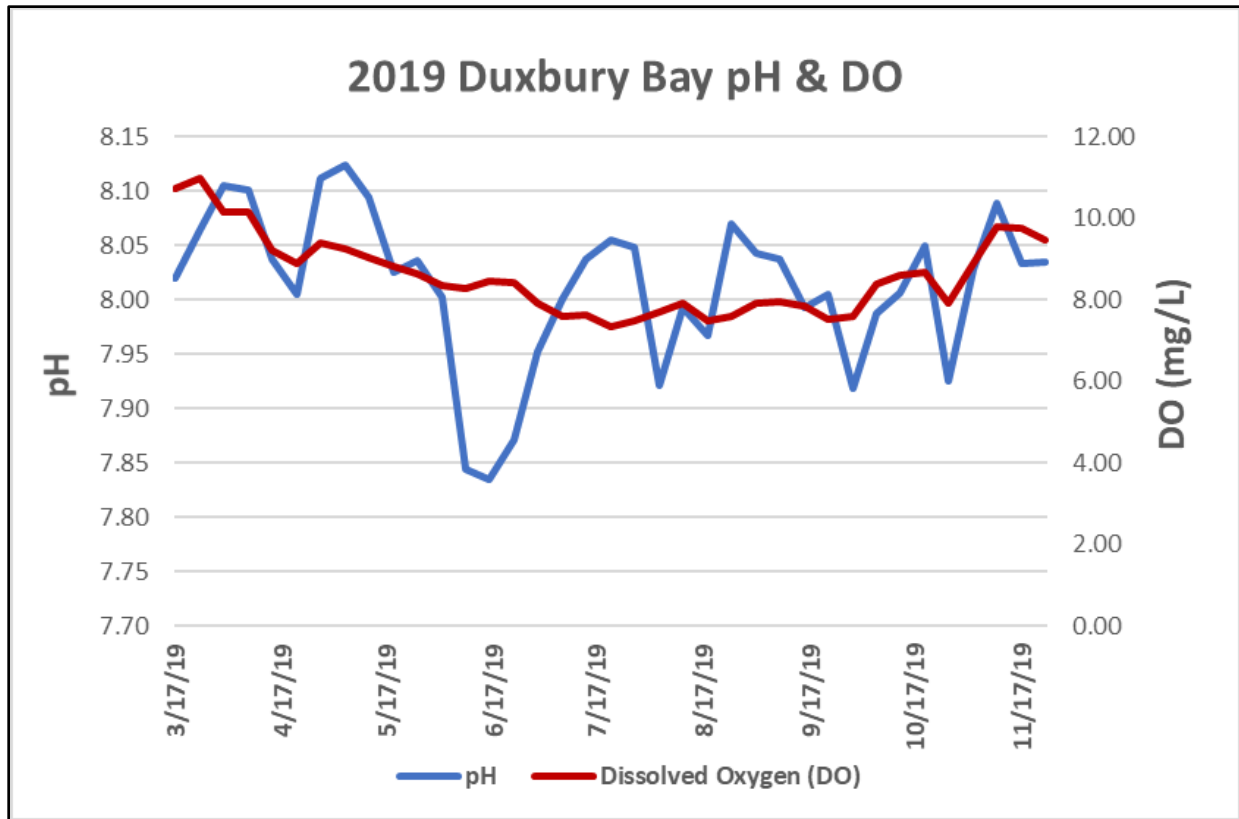
Weekly mean pH and dissolved oxygen as measured in Duxbury Bay during 2019.
