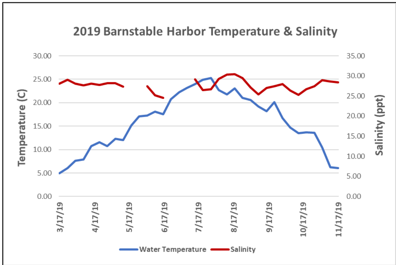
Weekly mean water temperature and salinity as measured at Scudders Landing in Barnstable Harbor during 2019.
