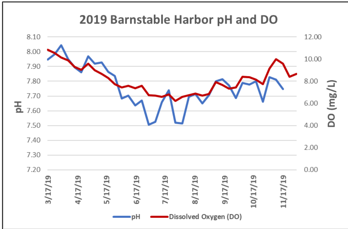
Weekly mean pH and dissolved oxygen as measured at Scudders Landing in Barnstable Harbor during 2019.
