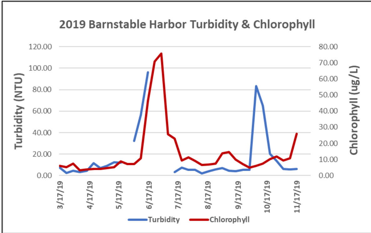
Weekly mean turbidity and chlorophyll as measured at Scudders Landing in Barnstable Harbor during 2019.
