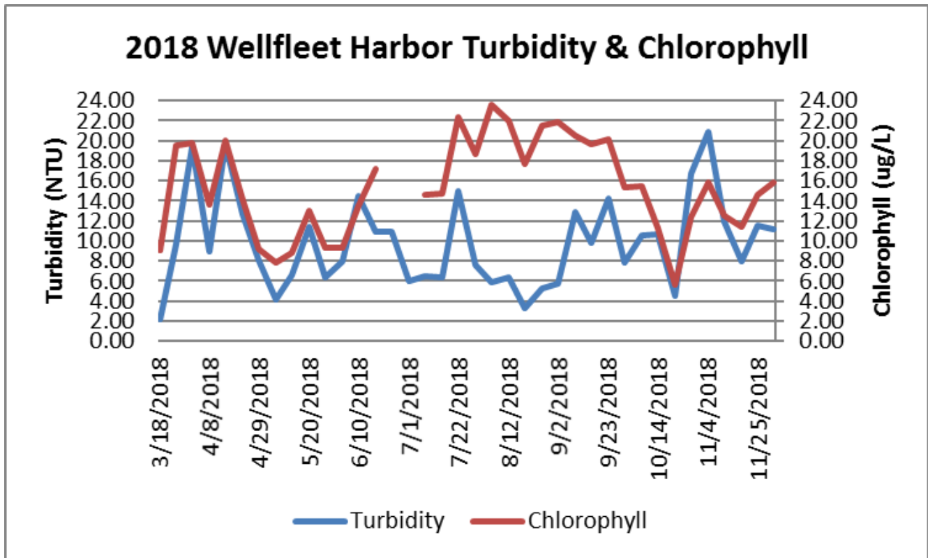
Weekly mean turbidity and chlorophyll as measured in Wellfleet Harbor during 2018.
