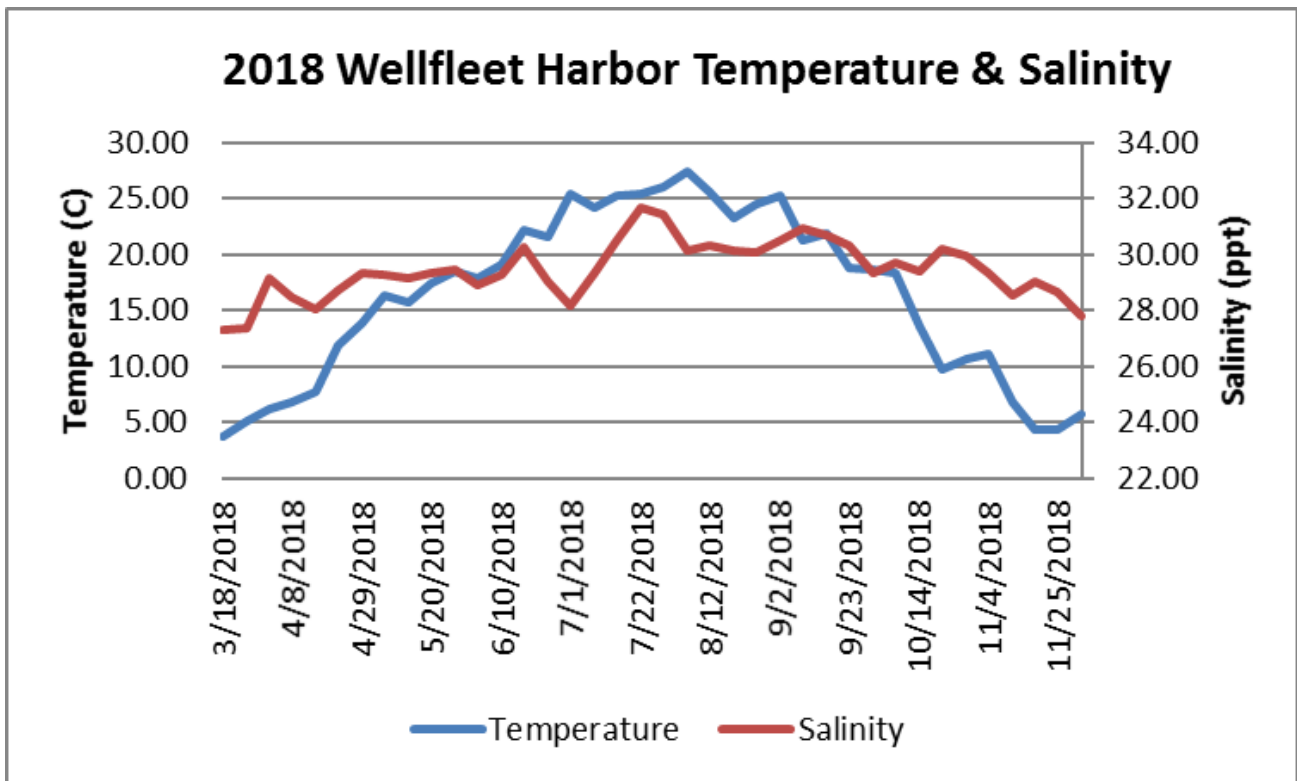
Weekly mean water temperature and salinity as measured in Wellfleet Harbor during 2018.
