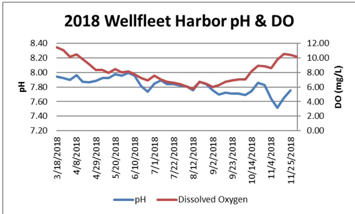
Weekly mean pH and dissolved oxygen as measured in Wellfleet Harbor during 2018.
