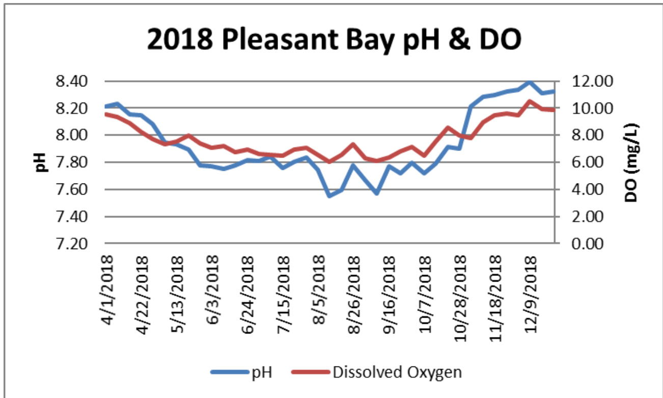
Weekly mean pH and dissolved oxygen as measured at Portanimicut Landing in Pleasant Bay during 2018.
