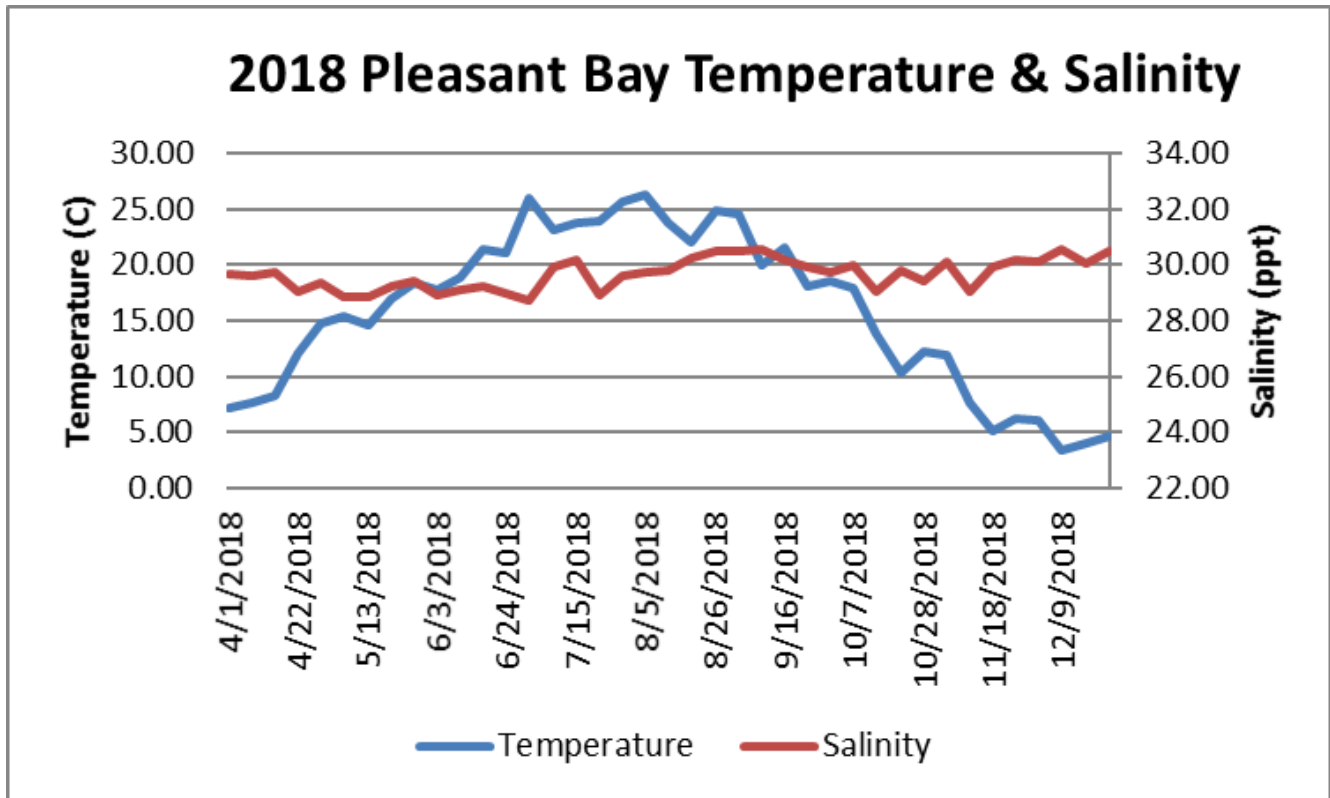
Weekly mean water temperature and salinity as measured at Portanimicut Landing in Pleasant Bay during 2018.
