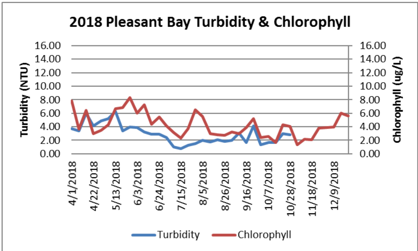
Weekly mean turbidity and chlorophyll as measured at Portanimicut Landing in Pleasant Bay during 2018.
