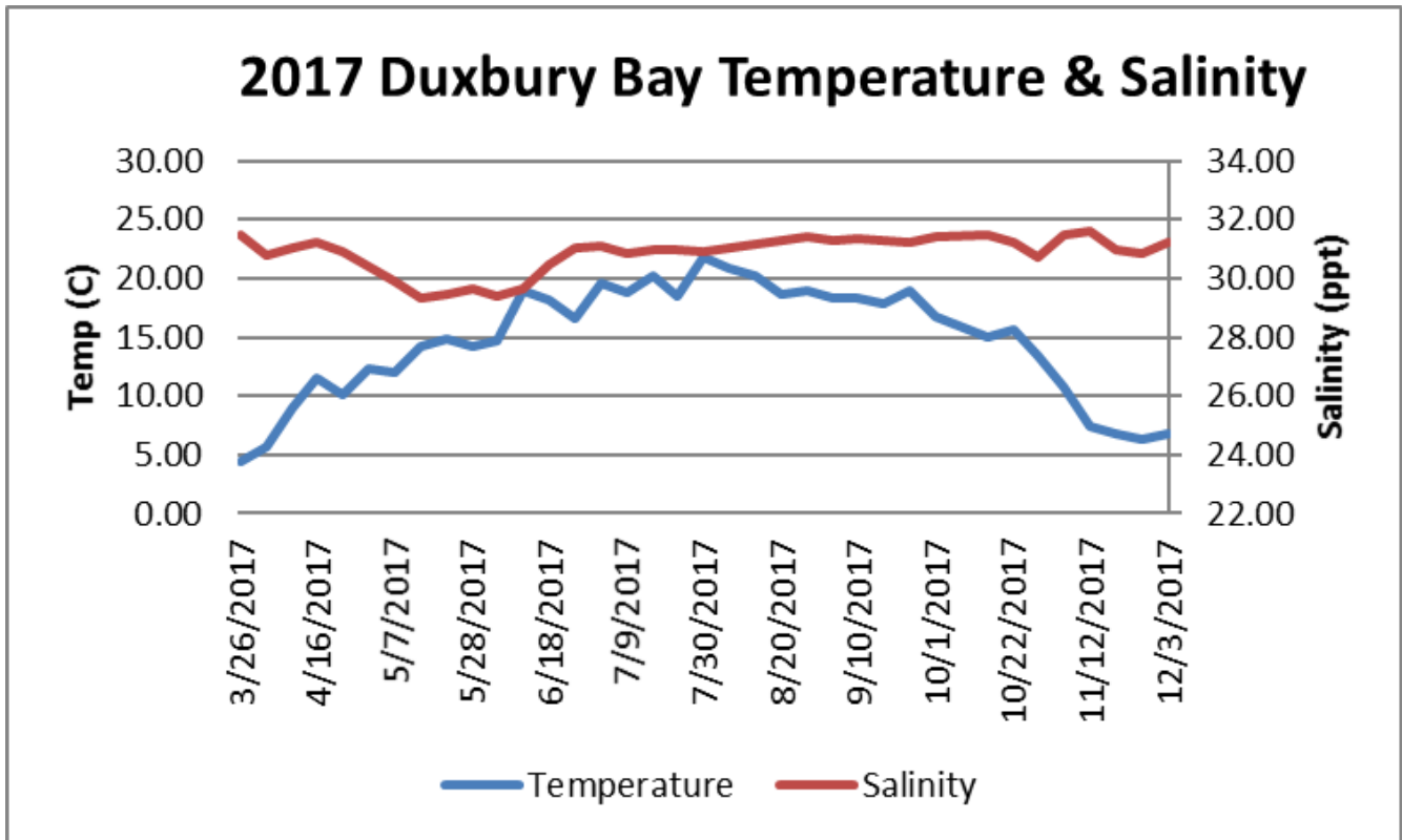
Weekly mean water temperature and salinity as measured in Duxbury Bay during 2017.
