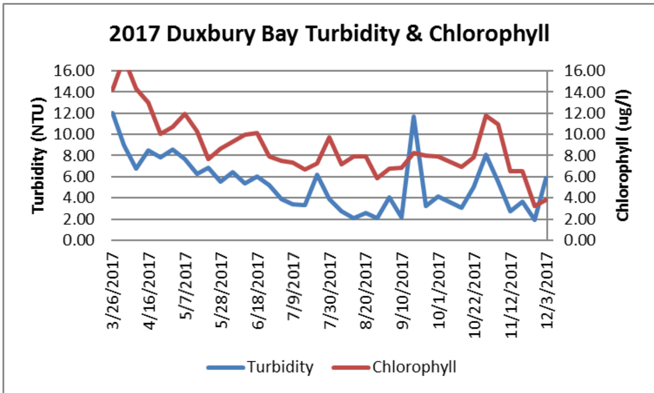
Weekly mean turbidity and chlorophyll as measured in Duxbury Bay during 2017.
