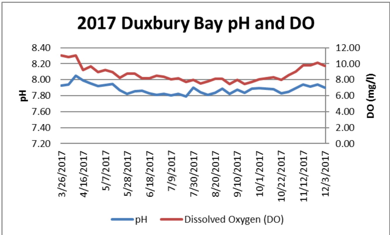
Weekly mean pH and dissolved oxygen as measured in Duxbury Bay during 2017.
