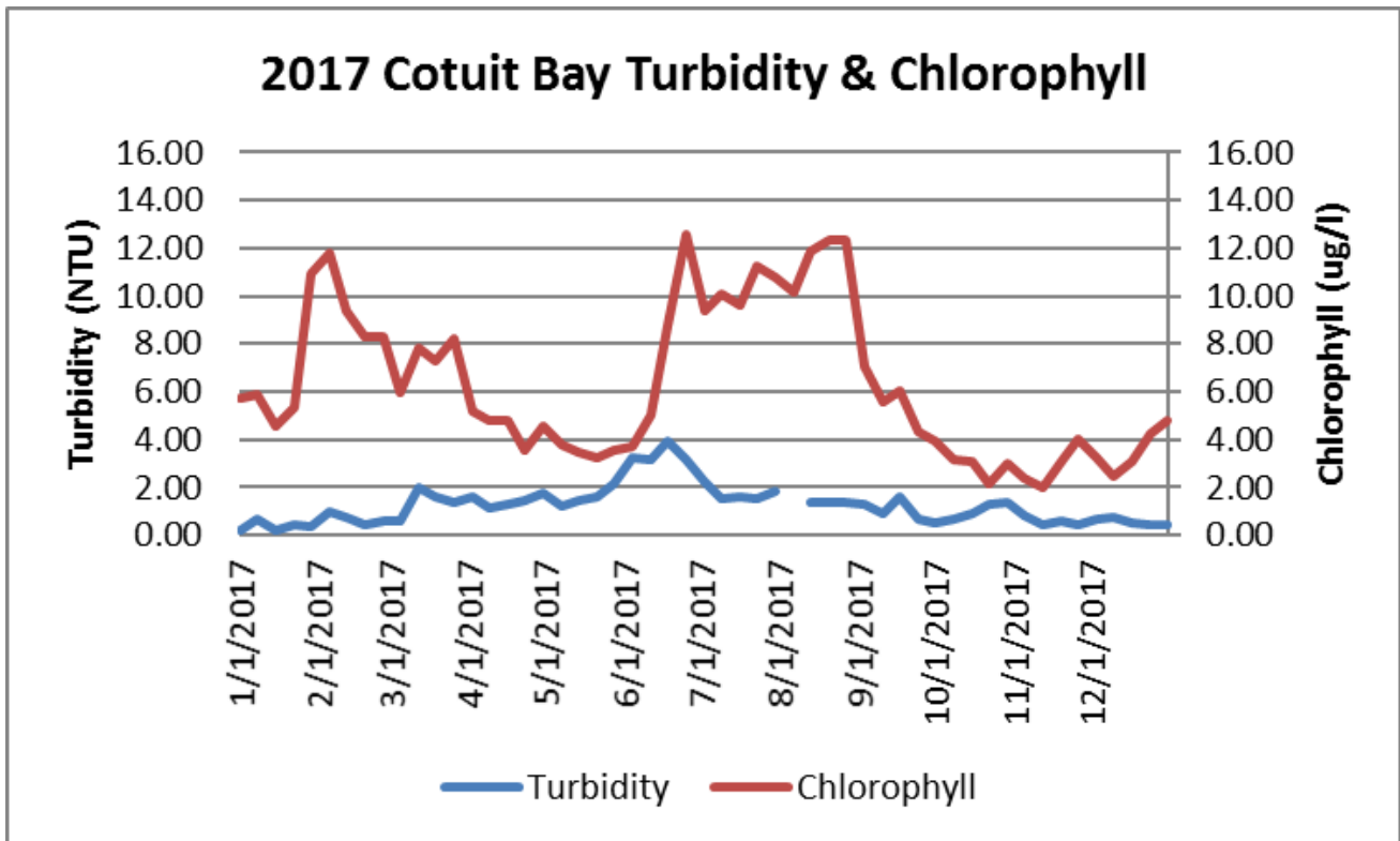
Weekly mean turbidity and chlorophyll as measured at Cotuit Bay during 2017.
