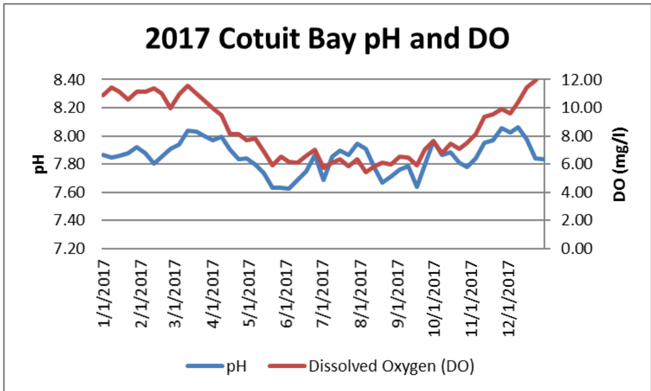
Weekly mean pH and dissolved oxygen as measured at Cotuit Bay during 2017.
