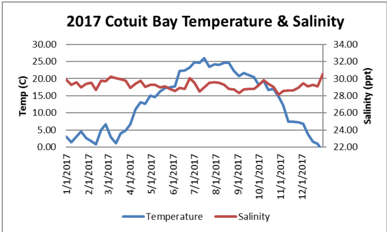
Weekly mean water temperature and salinity as measured at Cotuit Bay during 2017.
