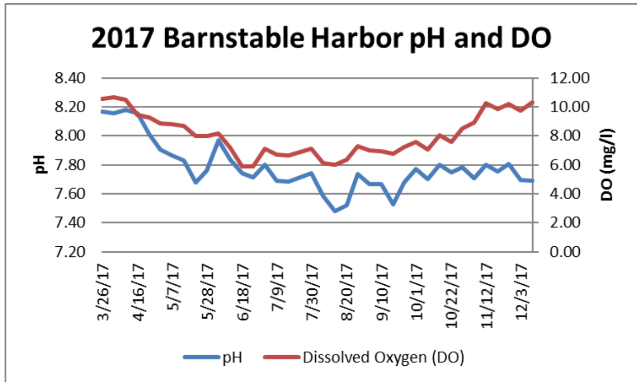
Weekly mean pH and dissolved oxygen as measured at Scudders Landing in Barnstable Harbor during 2017.
