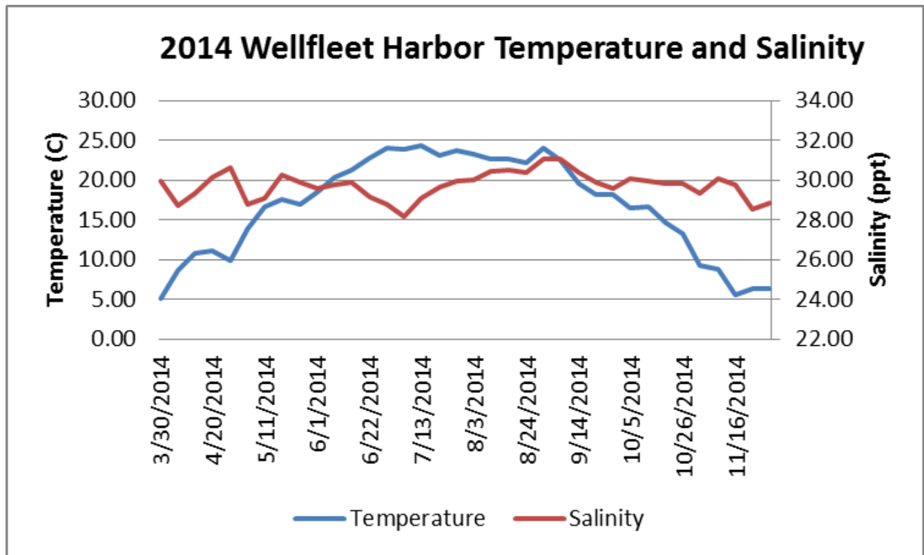
Weekly mean water temperature and salinity as measured in Wellfleet Harbor during 2014.
