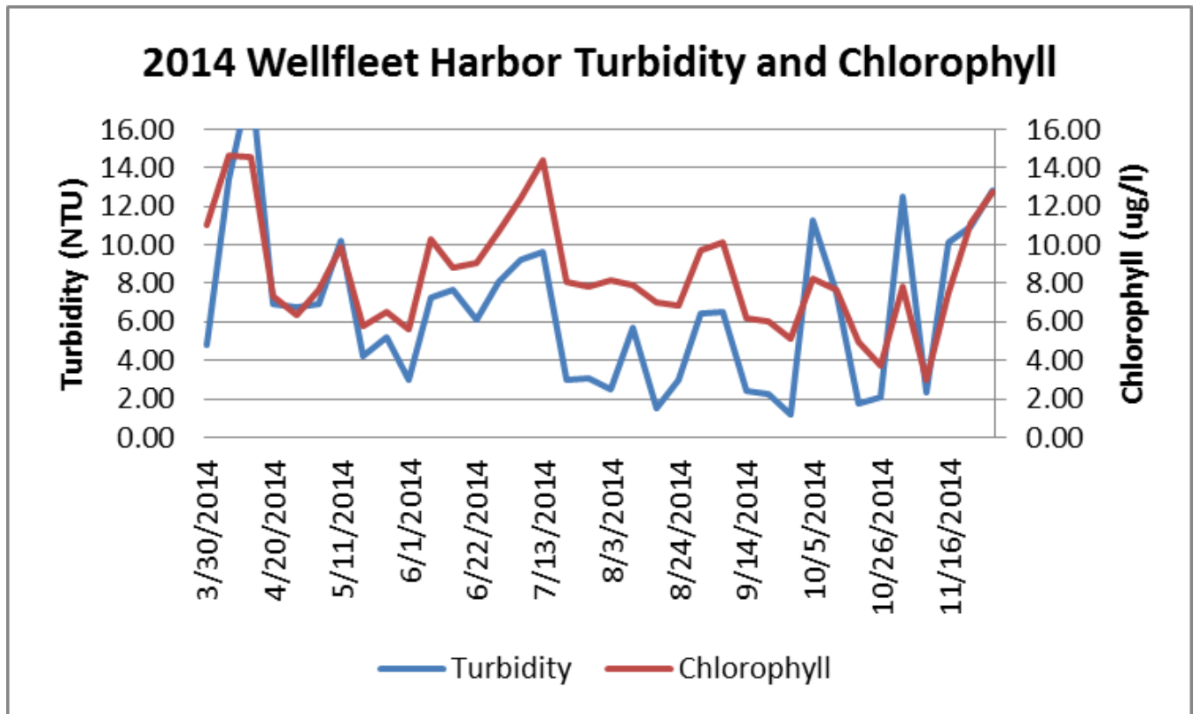
Weekly mean turbidity and chlorophyll as measured in Wellfleet Harbor during 2014.
