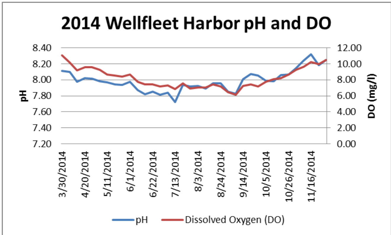
Weekly mean pH and dissolved oxygen as measured in Wellfleet Harbor during 2014.
