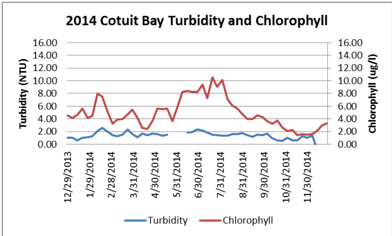
Weekly mean turbidity and chlorophyll as measured at Cotuit Bay during 2014.
