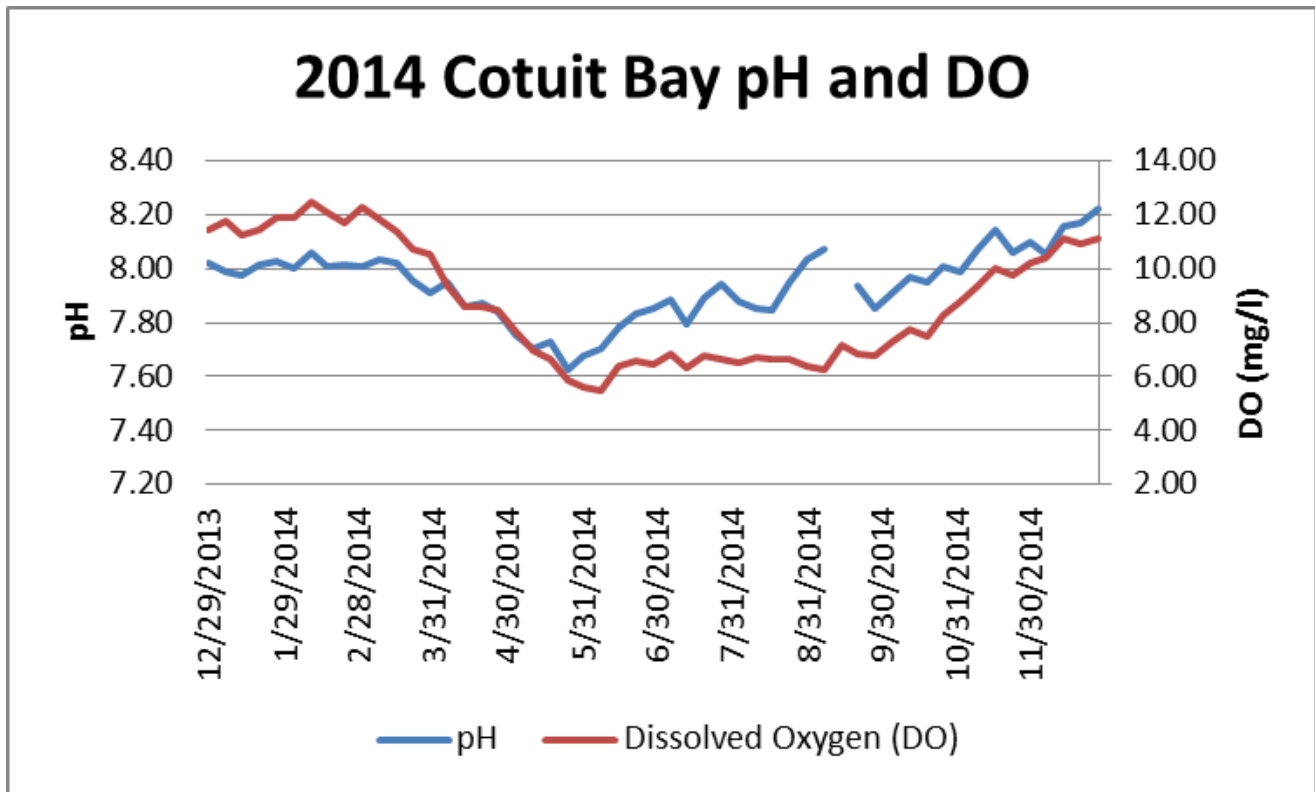
Weekly mean pH and dissolved oxygen as measured at Cotuit Bay during 2014.
