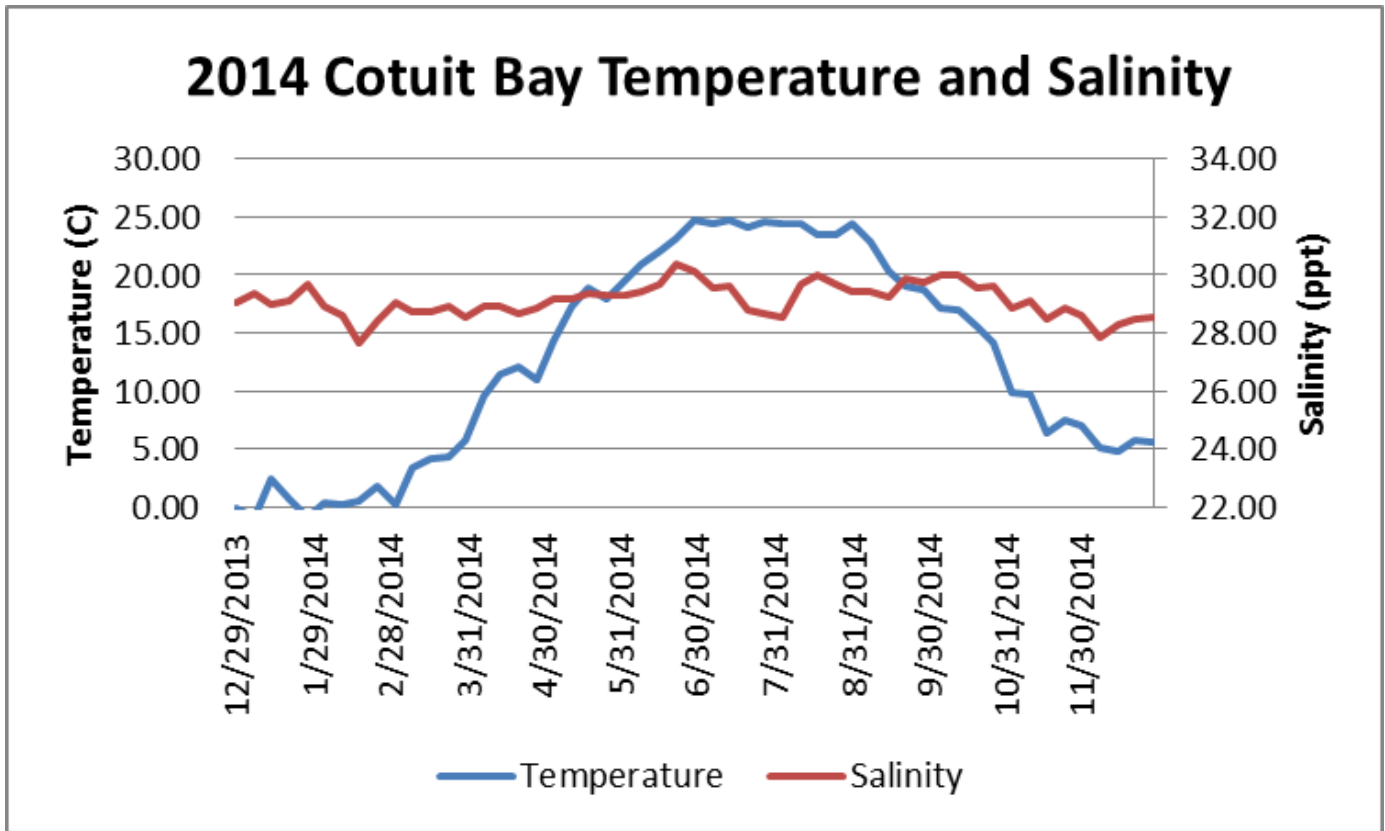
Weekly mean water temperature and salinity as measured at Cotuit Bay during 2014.
