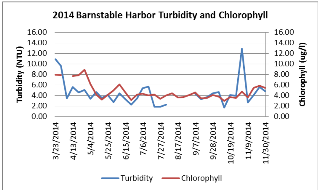
Weekly mean turbidity and chlorophyll as measured at Scudders Landing in Barnstable Harbor during 2014.
