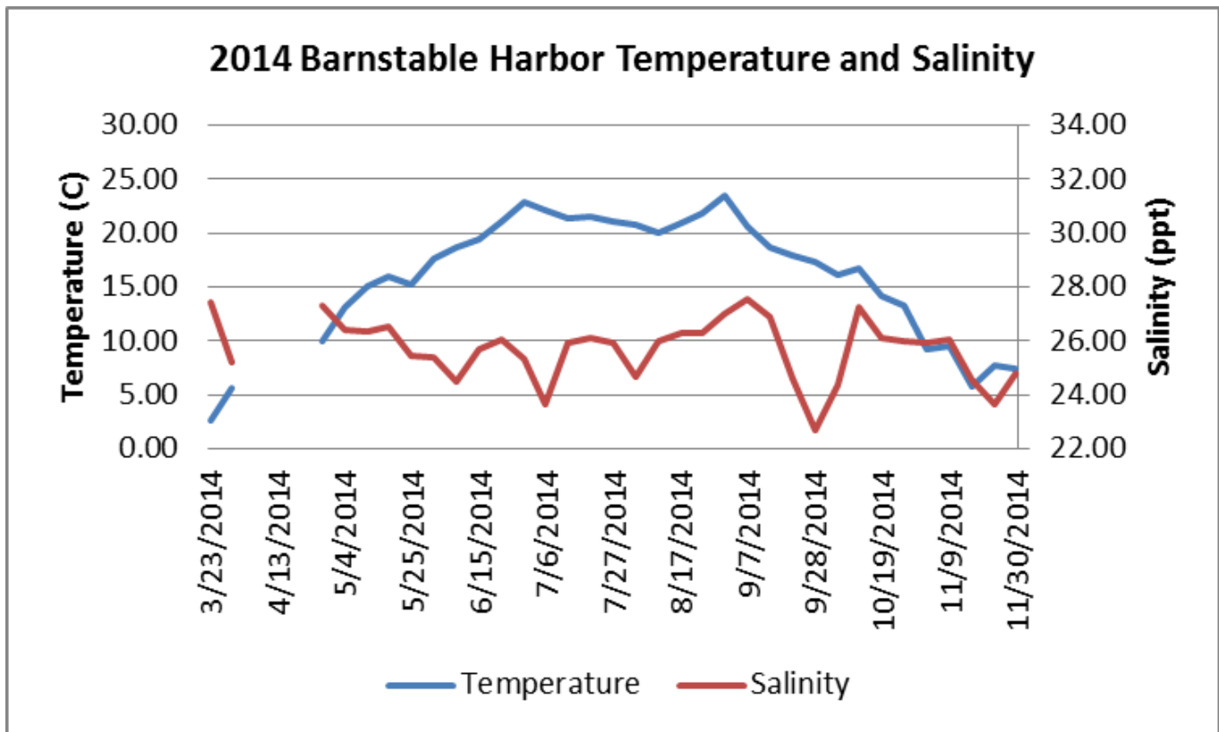
Weekly mean water temperature and salinity as measured at Scudders Landing in Barnstable Harbor during 2014.
