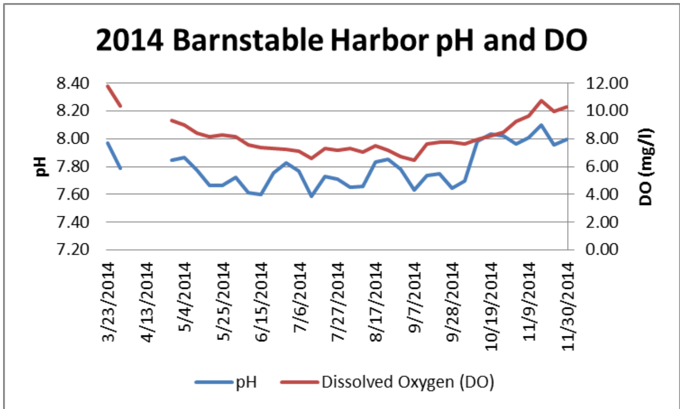
Weekly mean pH and dissolved oxygen as measured at Scudders Landing in Barnstable Harbor during 2014.
