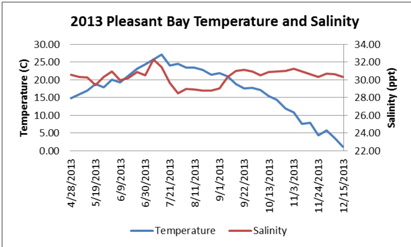
Weekly mean water temperature and salinity as measured at Portanimicut Landing in Pleasant Bay during 2013.
