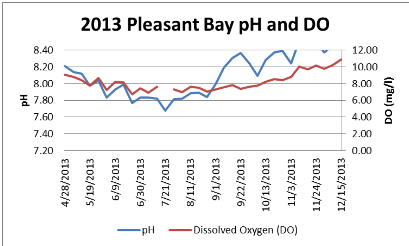
Weekly mean pH and dissolved oxygen as measured at Portanimicut Landing in Pleasant Bay during 2013.
