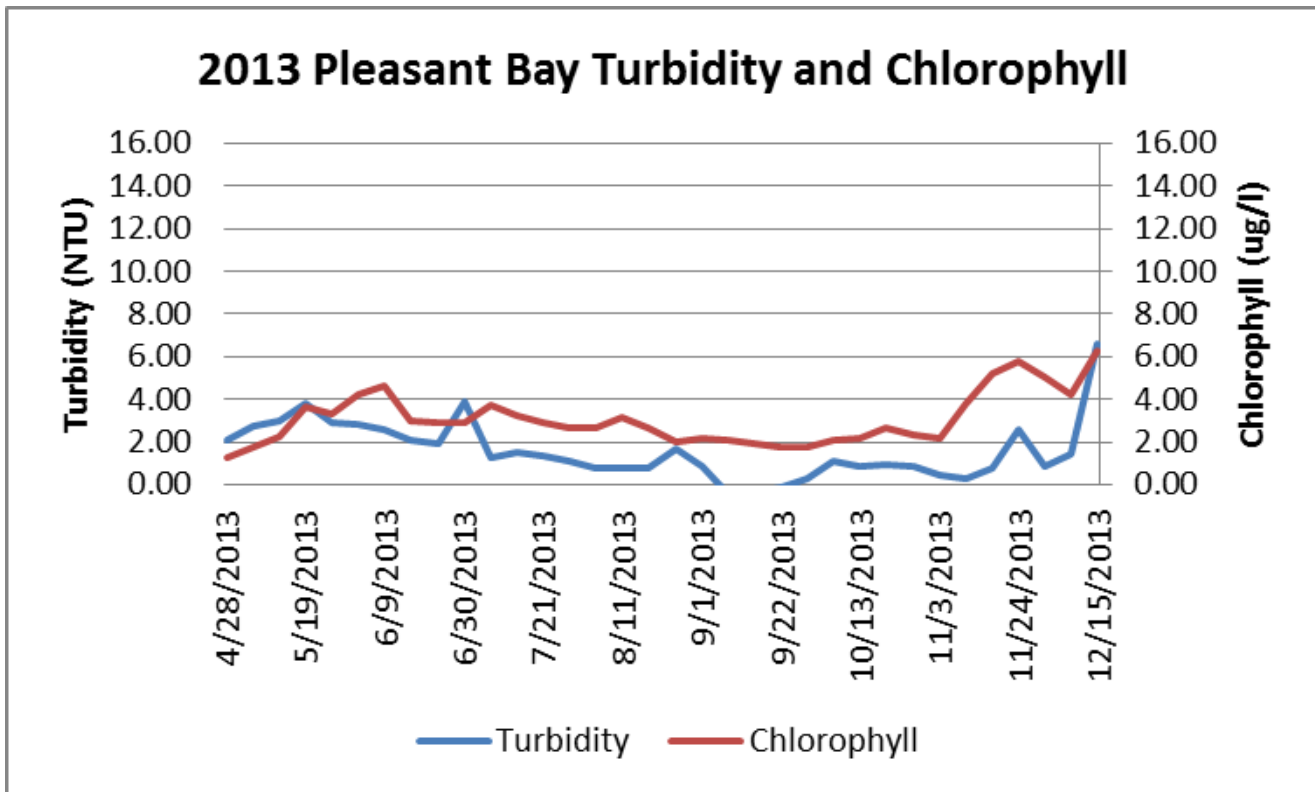
Weekly mean turbidity and chlorophyll as measured at Portanimicut Landing in Pleasant Bay during 2013.
