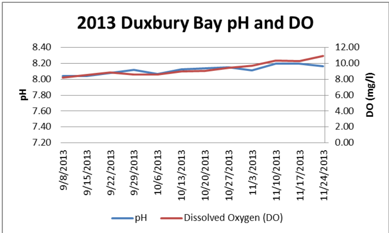
Weekly mean pH and dissolved oxygen as measured in Duxbury Bay during 2013.
