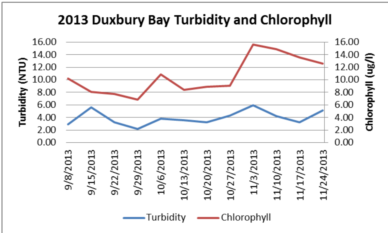
Weekly mean turbidity and chlorophyll as measured in Duxbury Bay during 2013.
