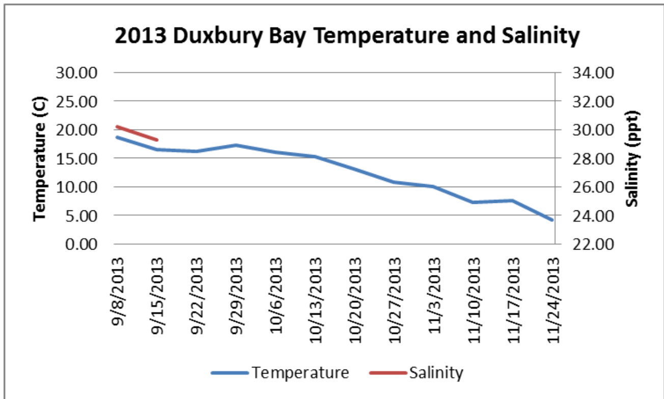
Weekly mean water temperature and salinity as measured in Duxbury Bay during 2013.
