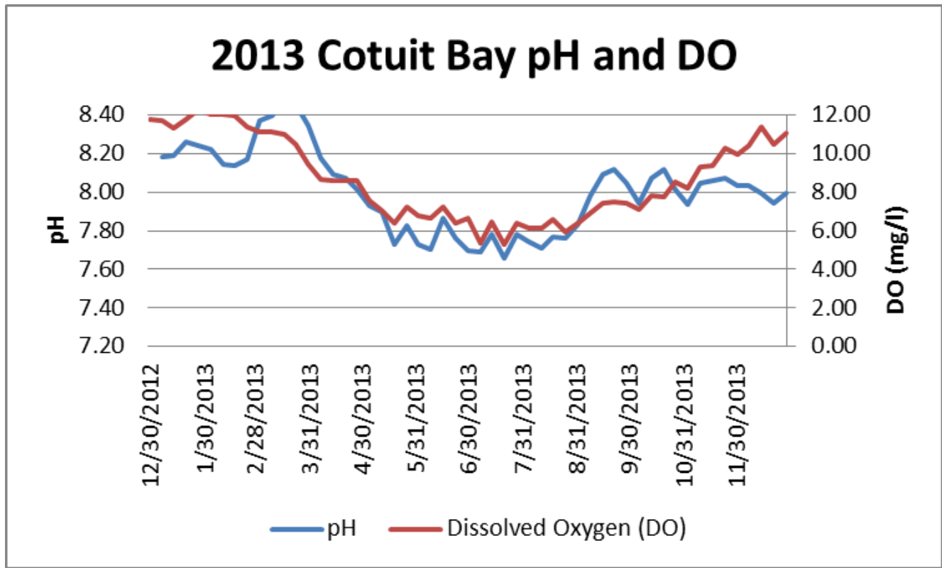
Weekly mean pH and dissolved oxygen as measured in Cotuit Bay during 2013.
