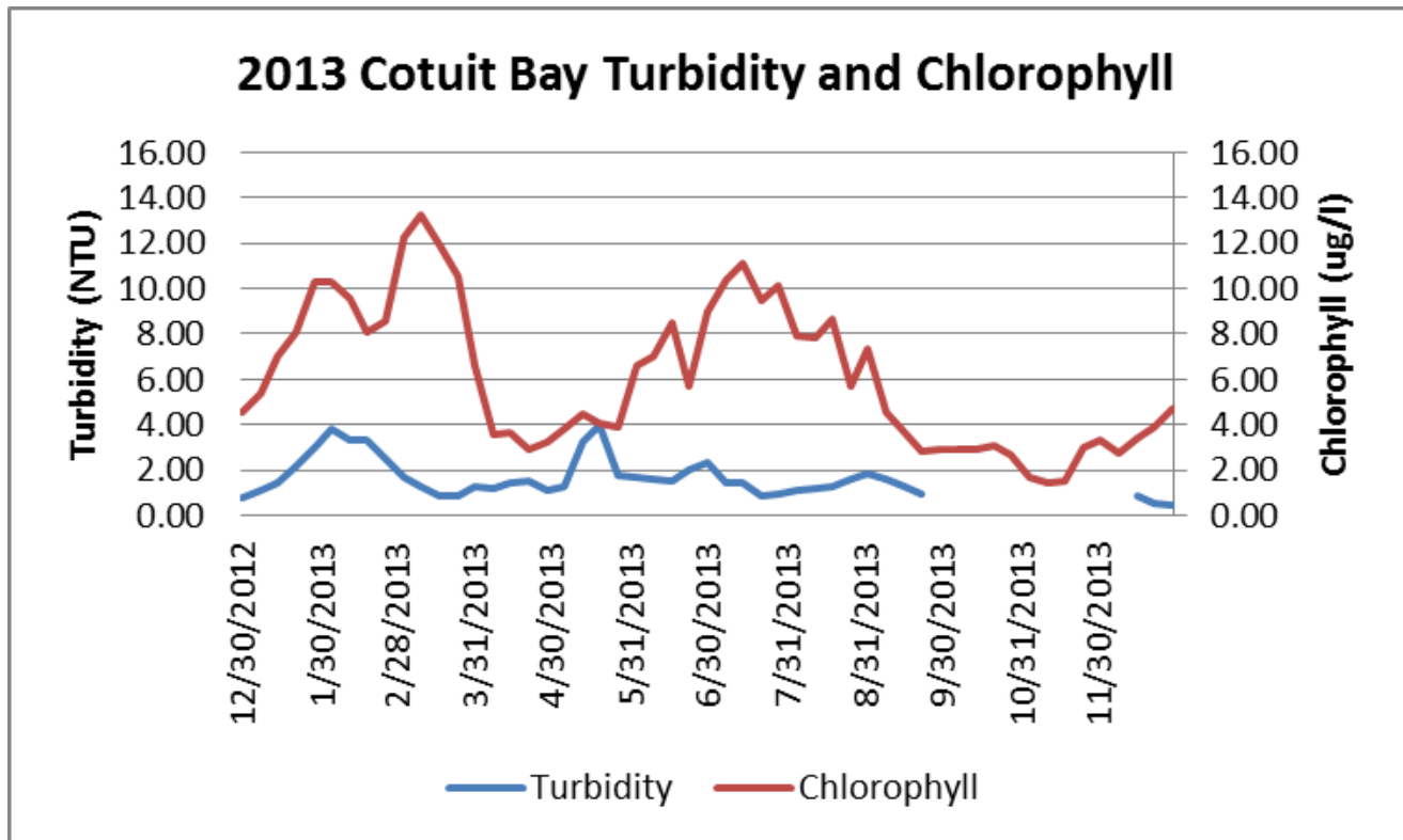
Weekly mean turbidity and chlorophyll as measured in Cotuit Bay during 2013.
