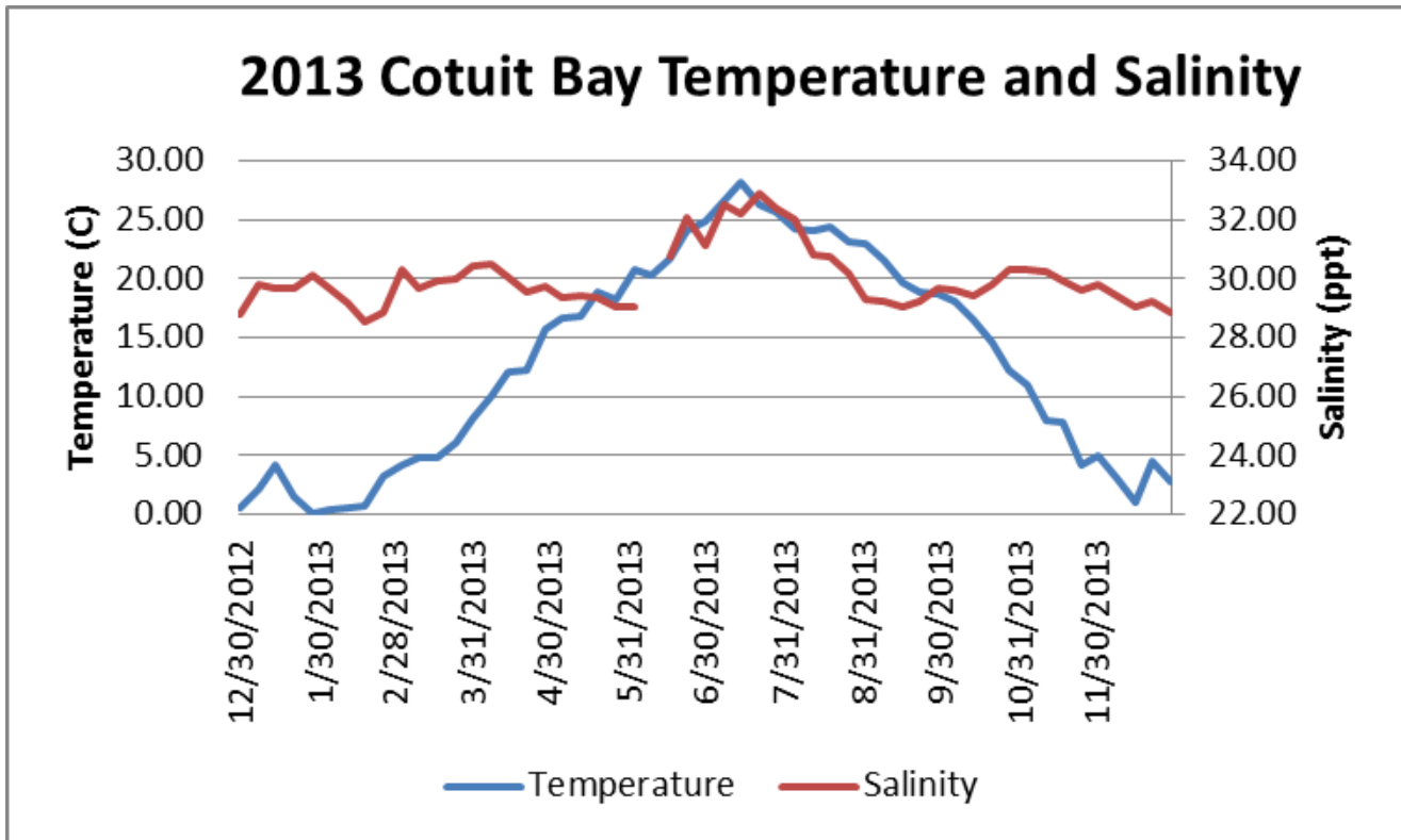
Weekly mean water temperature and salinity as measured in Cotuit Bay during 2013.
