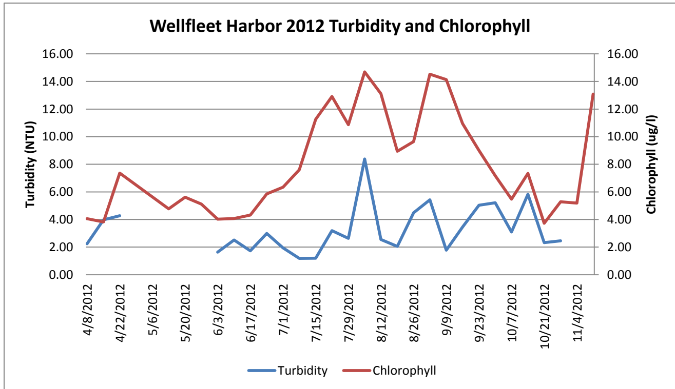
Weekly mean turbidity and chlorophyll as measured in Wellfleet Harbor during 2012.
