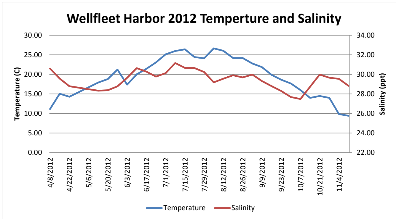
Weekly mean water temperature and salinity as measured in Wellfleet Harbor during 2012.
