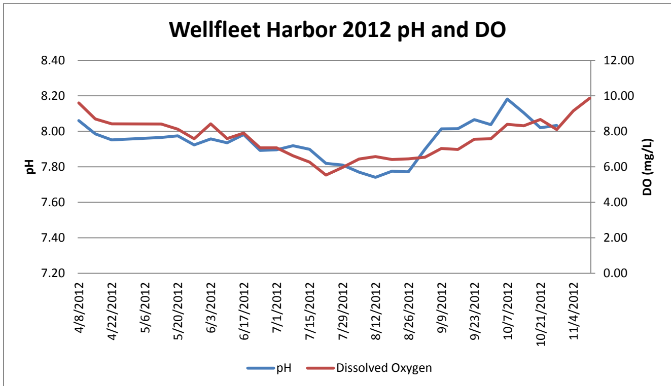
Weekly mean pH and dissolved oxygen as measured in Wellfleet Harbor during 2012.
