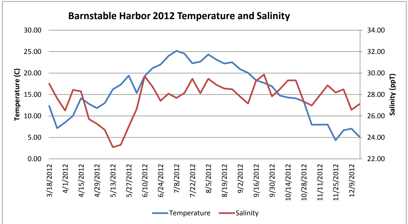
Weekly mean water temperature and salinity as measured at Scudders Landing in Barnstable Harbor during 2012.
