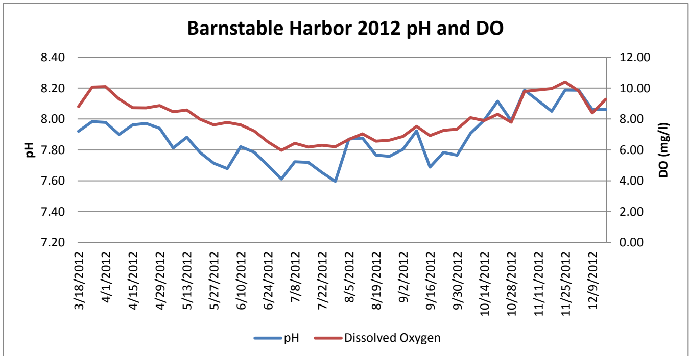
Weekly mean pH and dissolved oxygen as measured at Scudders Landing in Barnstable Harbor during 2012.
