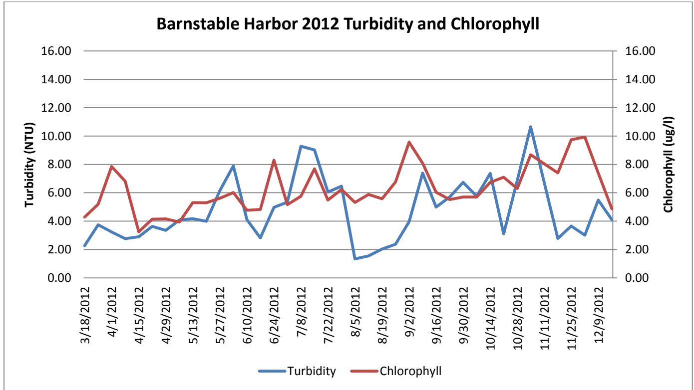
Weekly mean turbidity and chlorophyll as measured at Scudders Landing in Barnstable Harbor during 2012.
