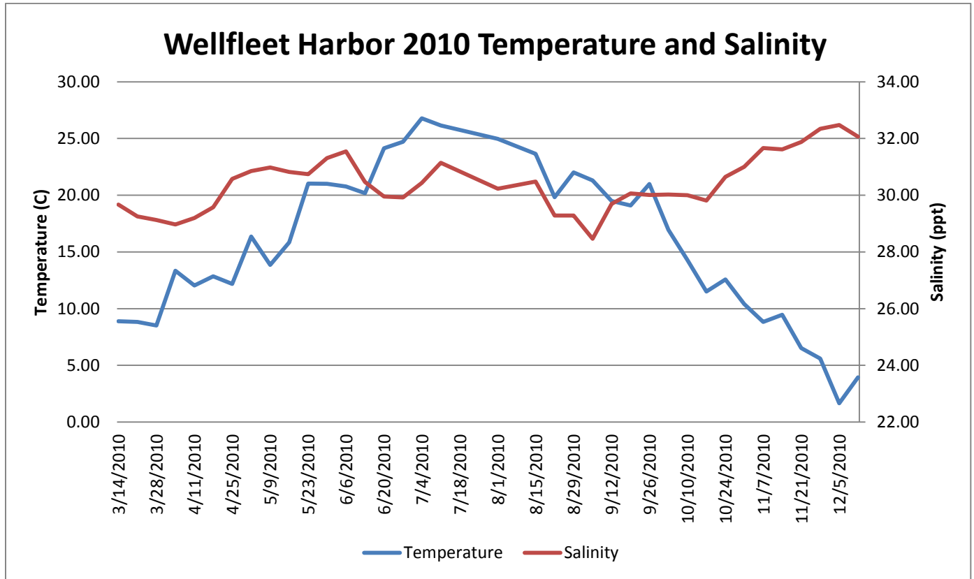
Weekly mean water temperature and salinity as measured in Wellfleet Harbor during 2010.
