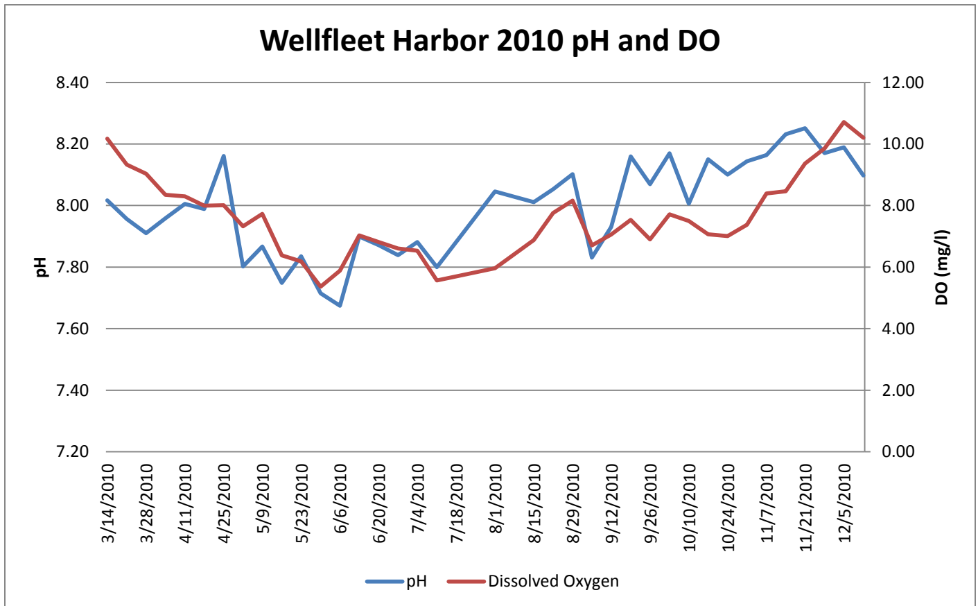
Weekly mean pH and dissolved oxygen as measured in Wellfleet Harbor during 2010.
