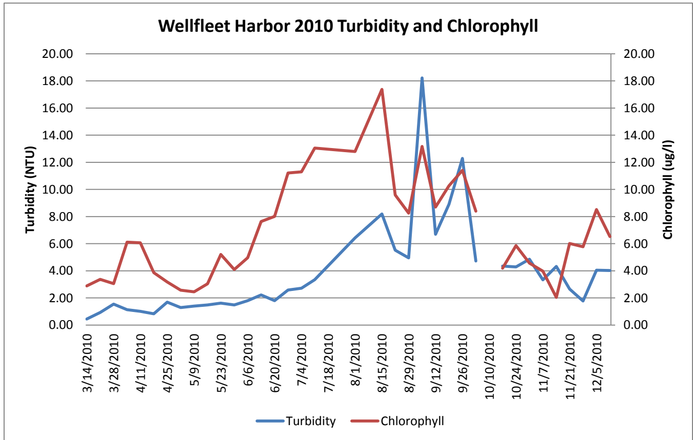
Weekly mean turbidity and chlorophyll as measured in Wellfleet Harbor during 2010.
