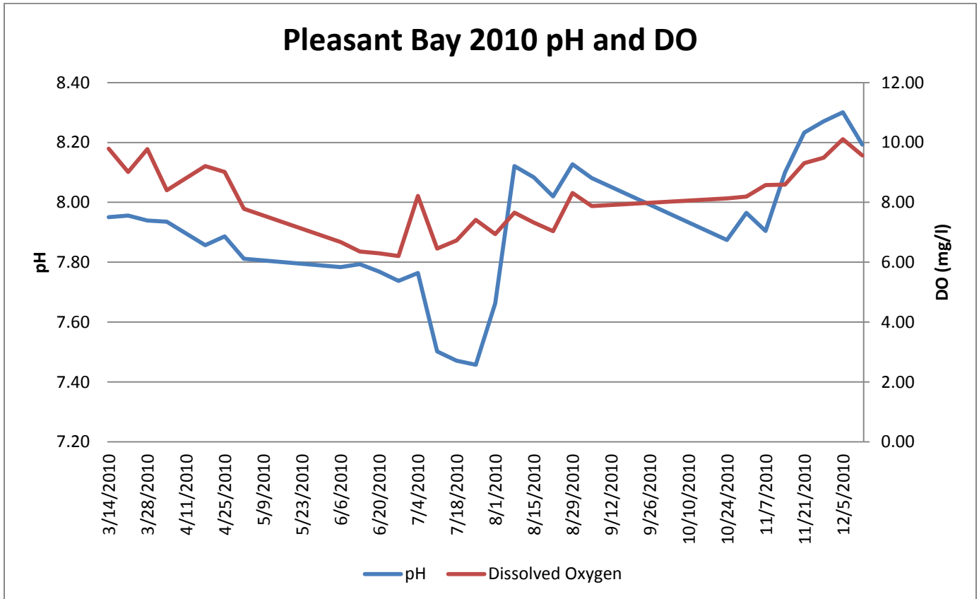
Weekly mean pH and dissolved oxygen as measured at Portanimicut Landing in Pleasant Bay during 2010.
