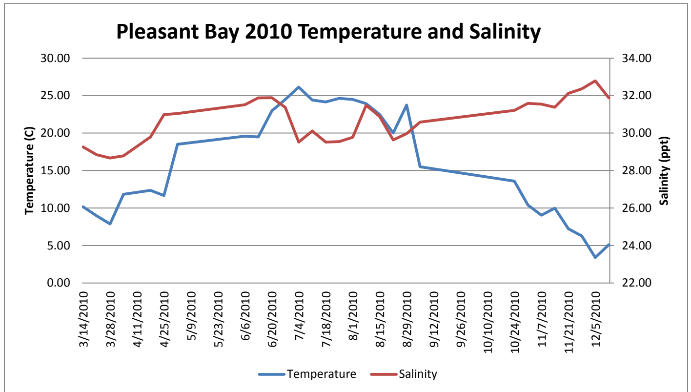
Weekly mean water temperature and salinity as measured at Portanimicut Landing in Pleasant Bay during 2010.
