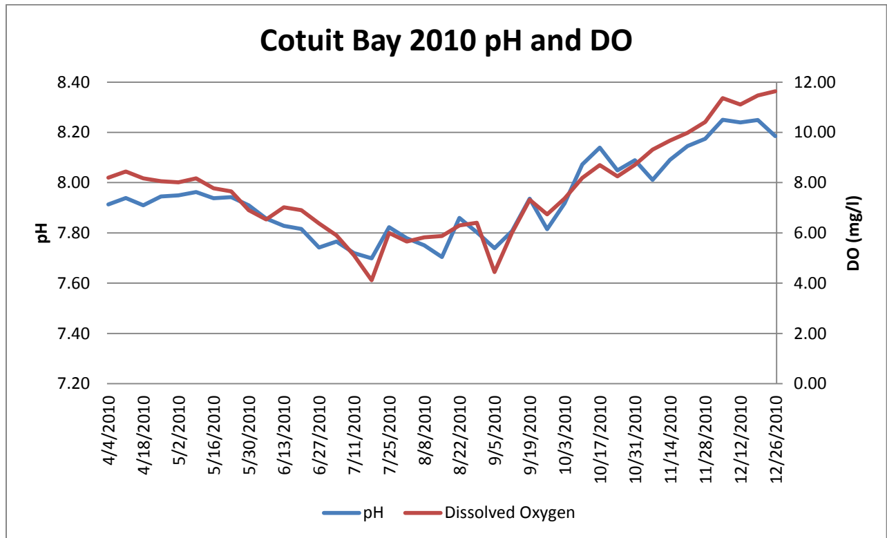
Weekly mean pH and dissolved oxygen as measured in Cotuit Bay during 2010.
