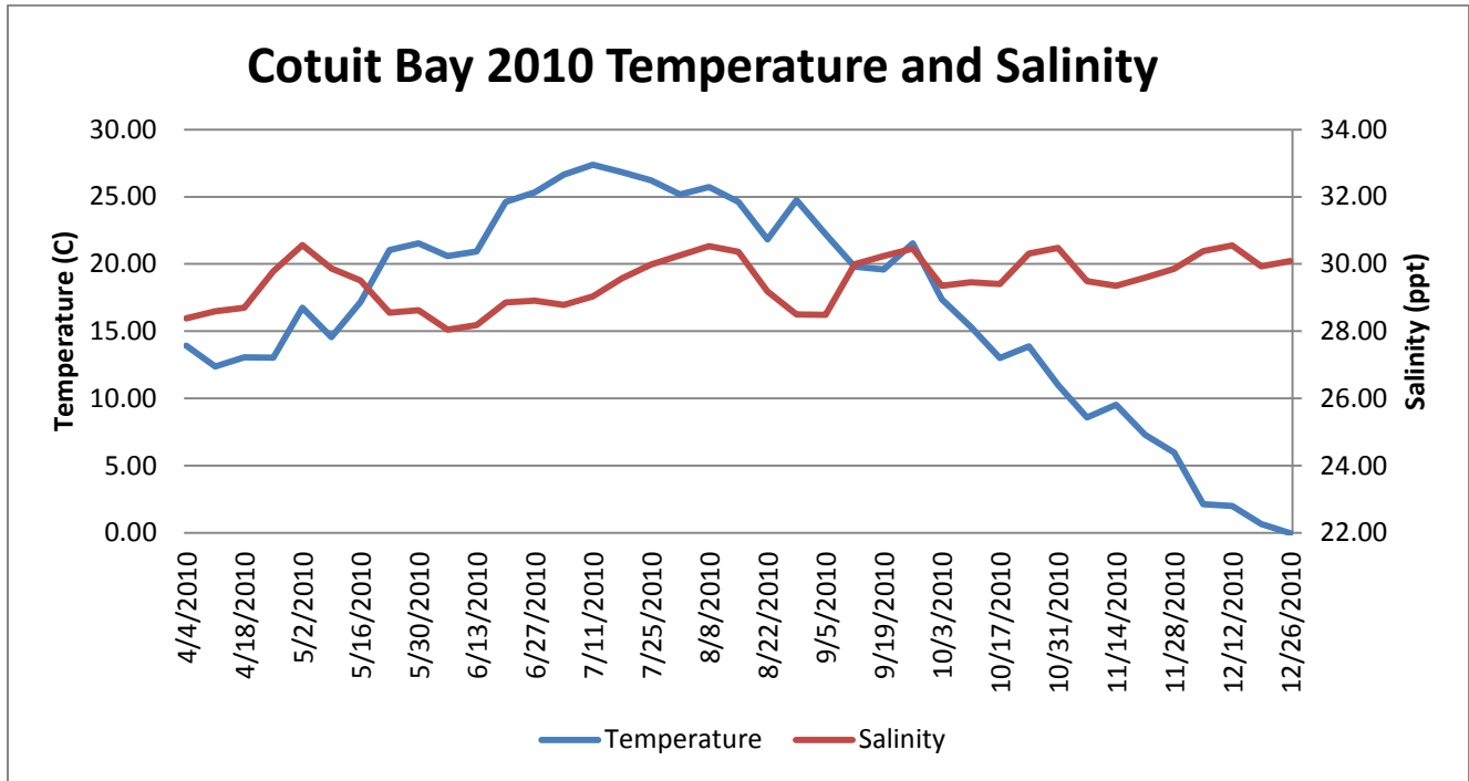
Weekly mean water temperature and salinity as measured in Cotuit Bay during 2010.
