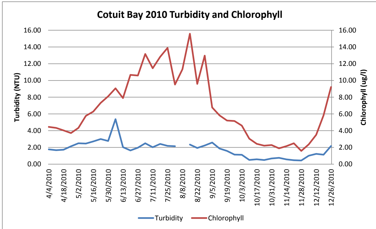
Weekly mean turbidity and chlorophyll as measured in Cotuit Bay during 2010.
