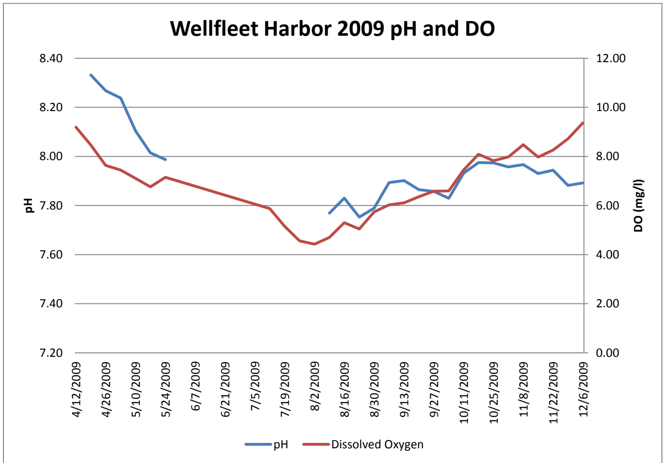
Weekly mean pH and dissolved oxygen as measured in Wellfleet Harbor during 2009.
