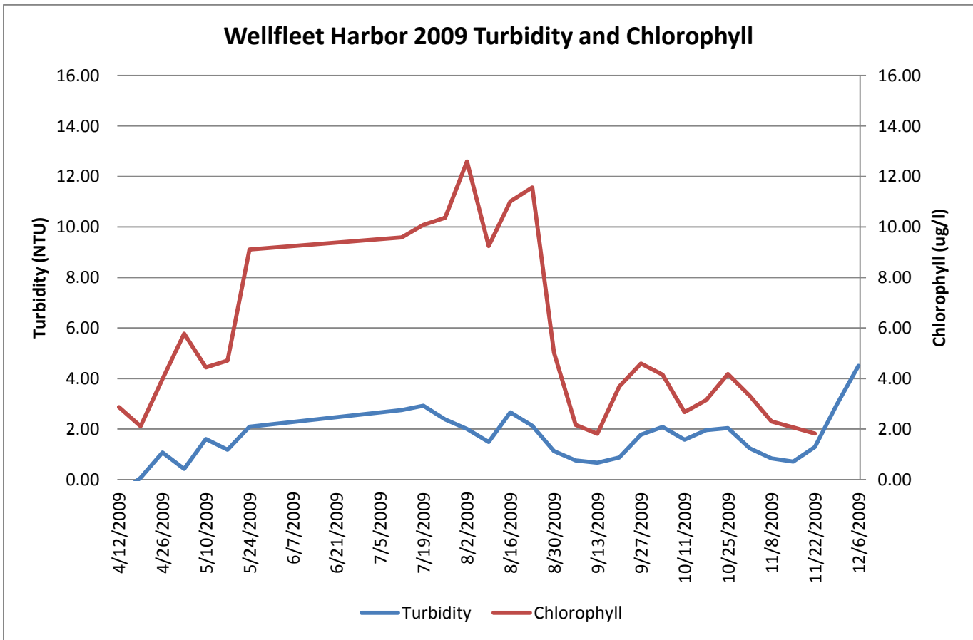
Weekly mean turbidity and chlorophyll as measured in Wellfleet Harbor during 2009.
