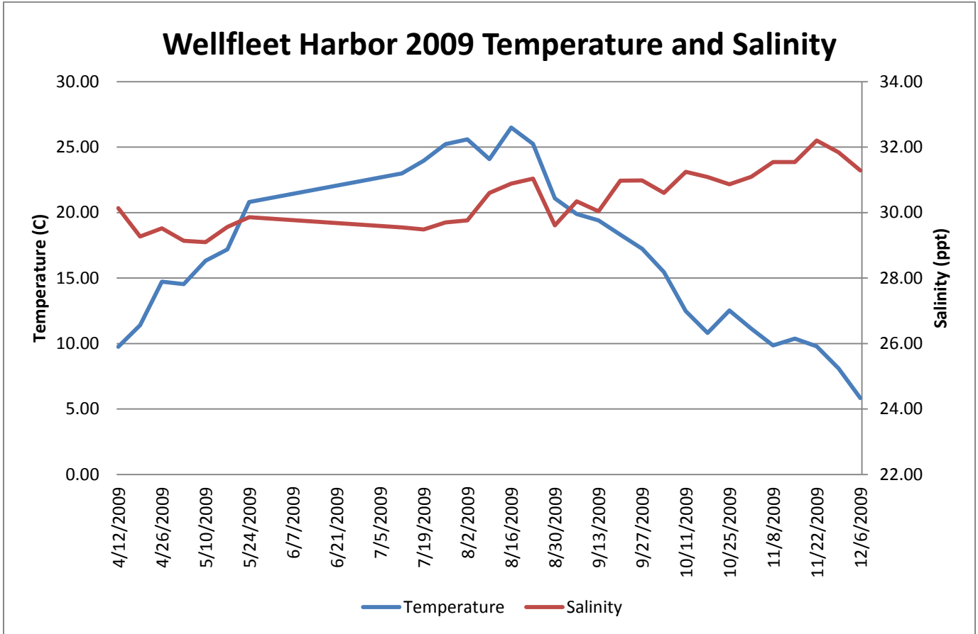
Weekly mean water temperature and salinity as measured in Wellfleet Harbor during 2009.
