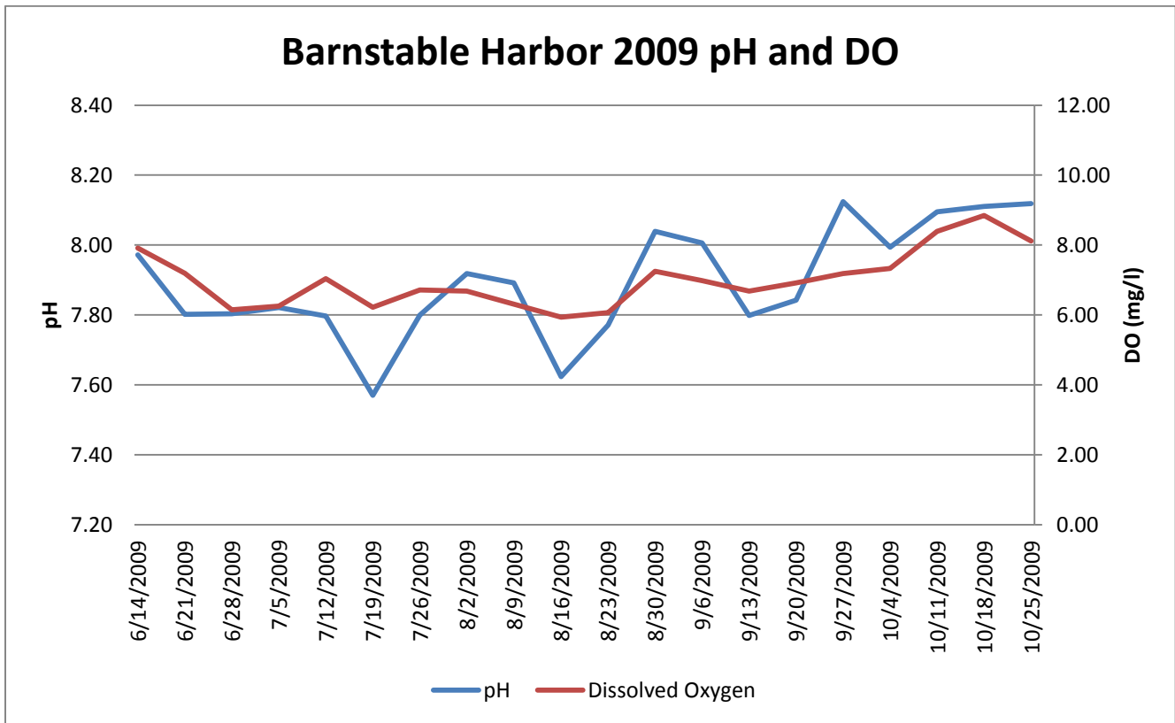
Weekly mean pH and dissolved oxygen as measured in Barnstable Harbor during 2009.
