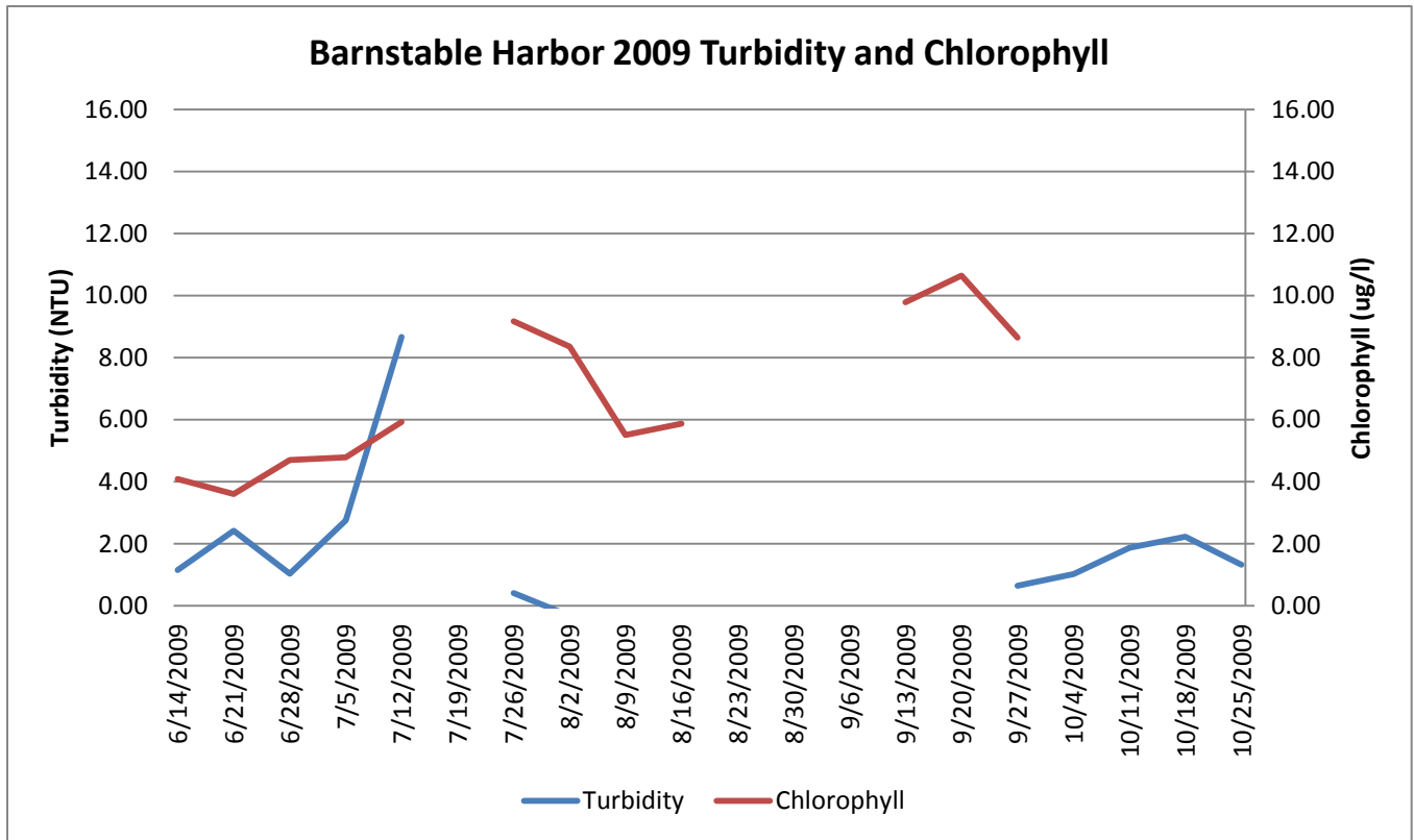
Weekly mean turbidity and chlorophyll as measured in Barnstable Harbor during 2009.
