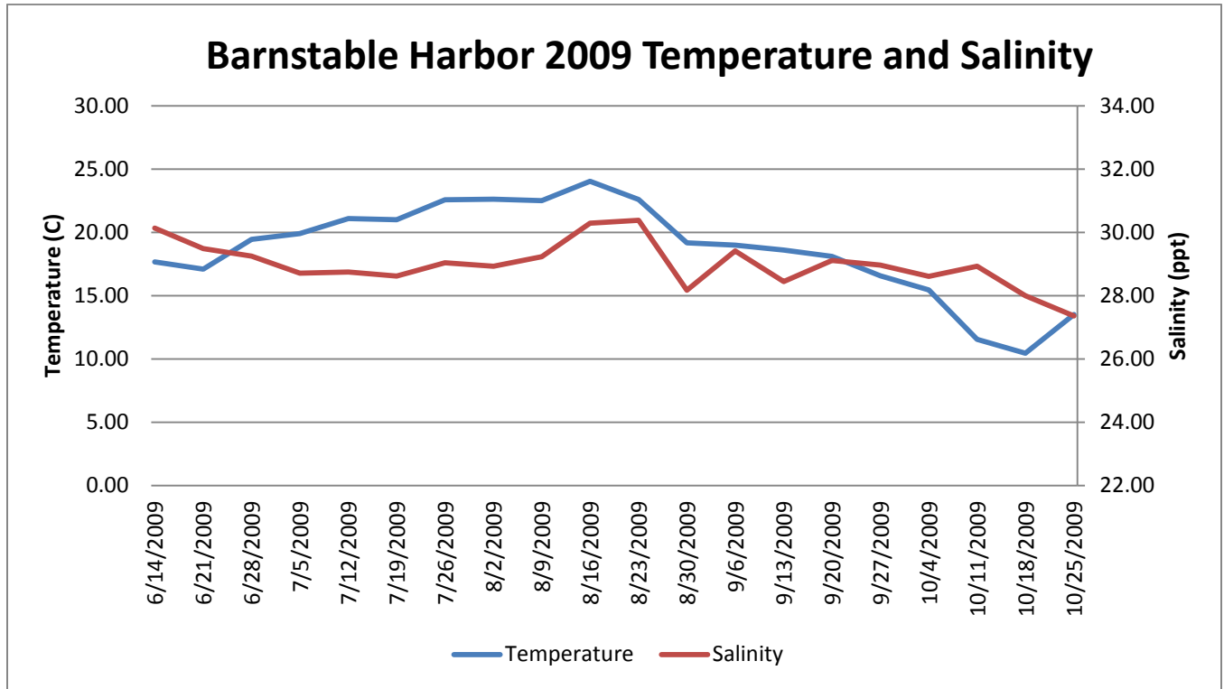
Weekly mean water temperature and salinity as measured in Barnstable Harbor during 2009.
