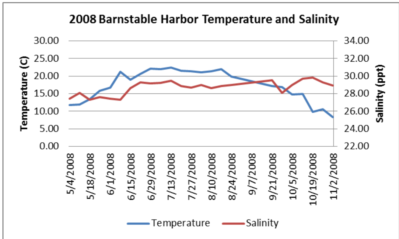
Weekly mean water temperature and salinity as measured at the Inner Harbor of Barnstable Harbor during 2008.
