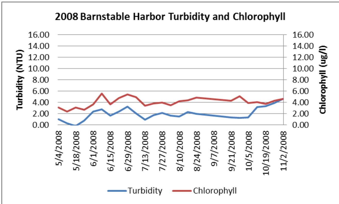
Weekly mean turbidity and chlorophyll as measured at the Inner Harbor of Barnstable Harbor during 2008.
