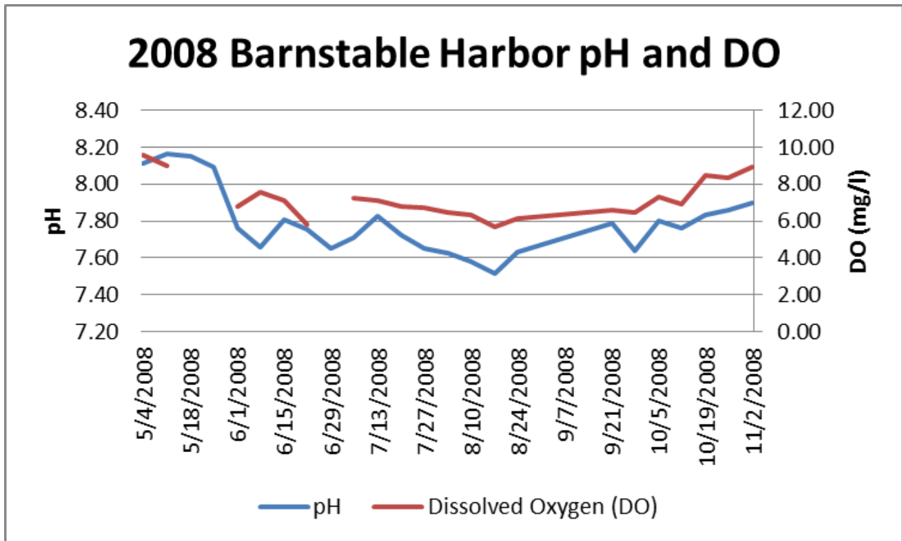
Weekly mean pH and dissolved oxygen as measured at the Inner Harbor of Barnstable Harbor during 2008.
