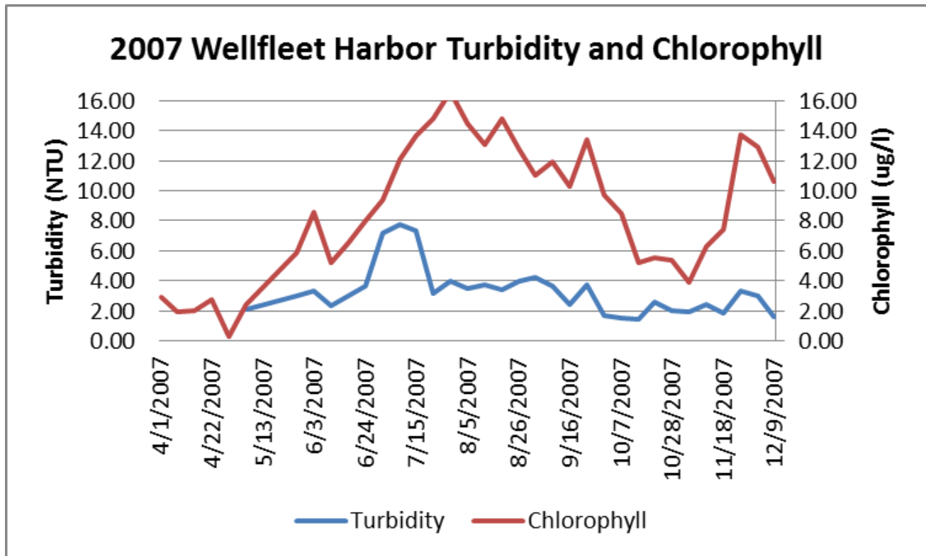
Weekly mean turbidity and chlorophyll as measured in Wellfleet Harbor during 2007.
