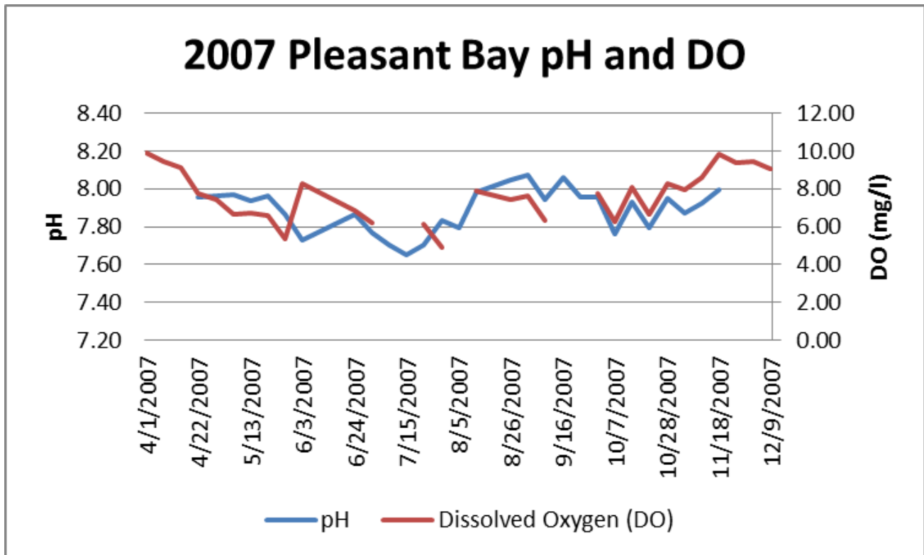
Weekly mean pH and dissolved oxygen as measured in Pleasant Bay at Portanimitcutt Landing during 2007.
