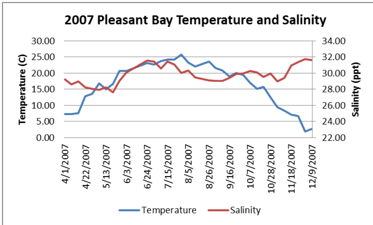
Weekly mean water temperature and salinity as measured in Pleasant Bay at Portanimicutt Landing during 2007.
