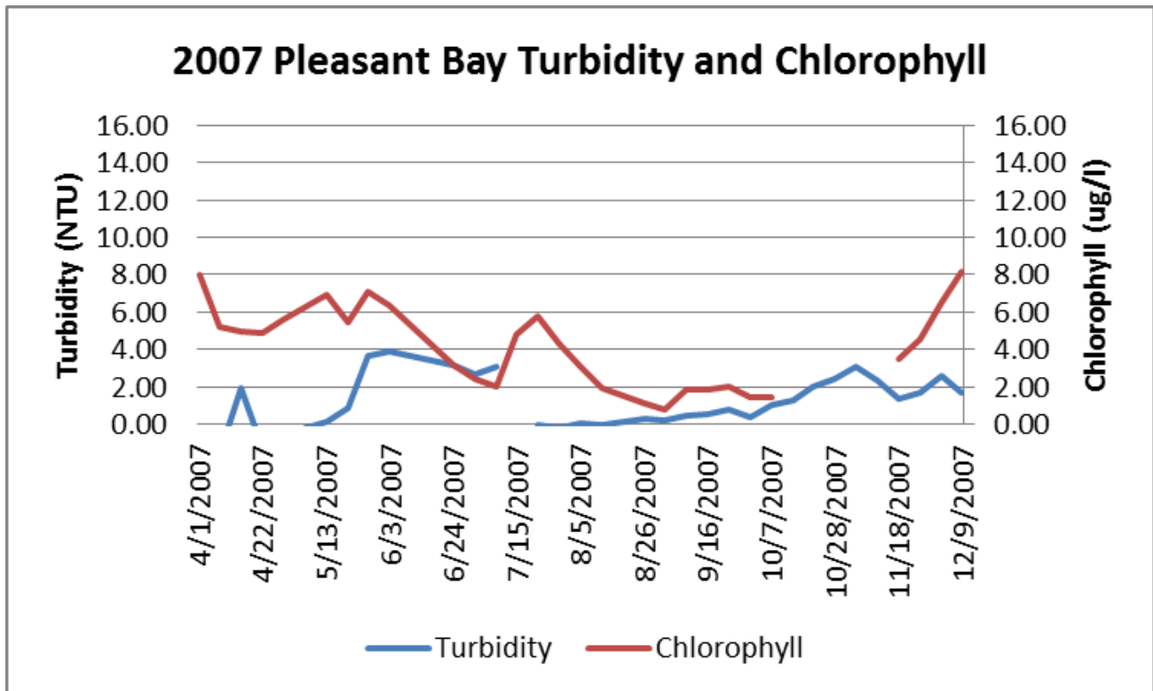
Weekly mean turbidity and chlorophyll as measured in Pleasant Bay at Portanimitcutt Landing during 2007.
