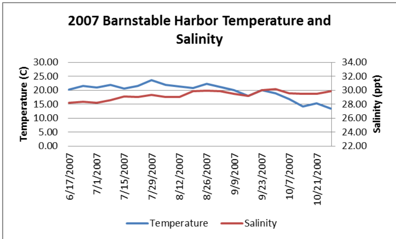
Weekly mean water temperature and salinity as measured at the Inner Harbor of Barnstable Harbor during 2007.
