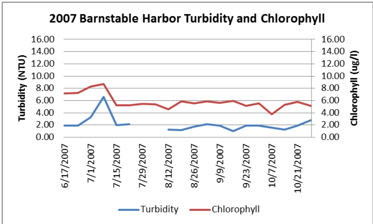
Weekly mean turbidity and chlorophyll as measured at the Inner Harbor of Barnstable Harbor during 2007.
