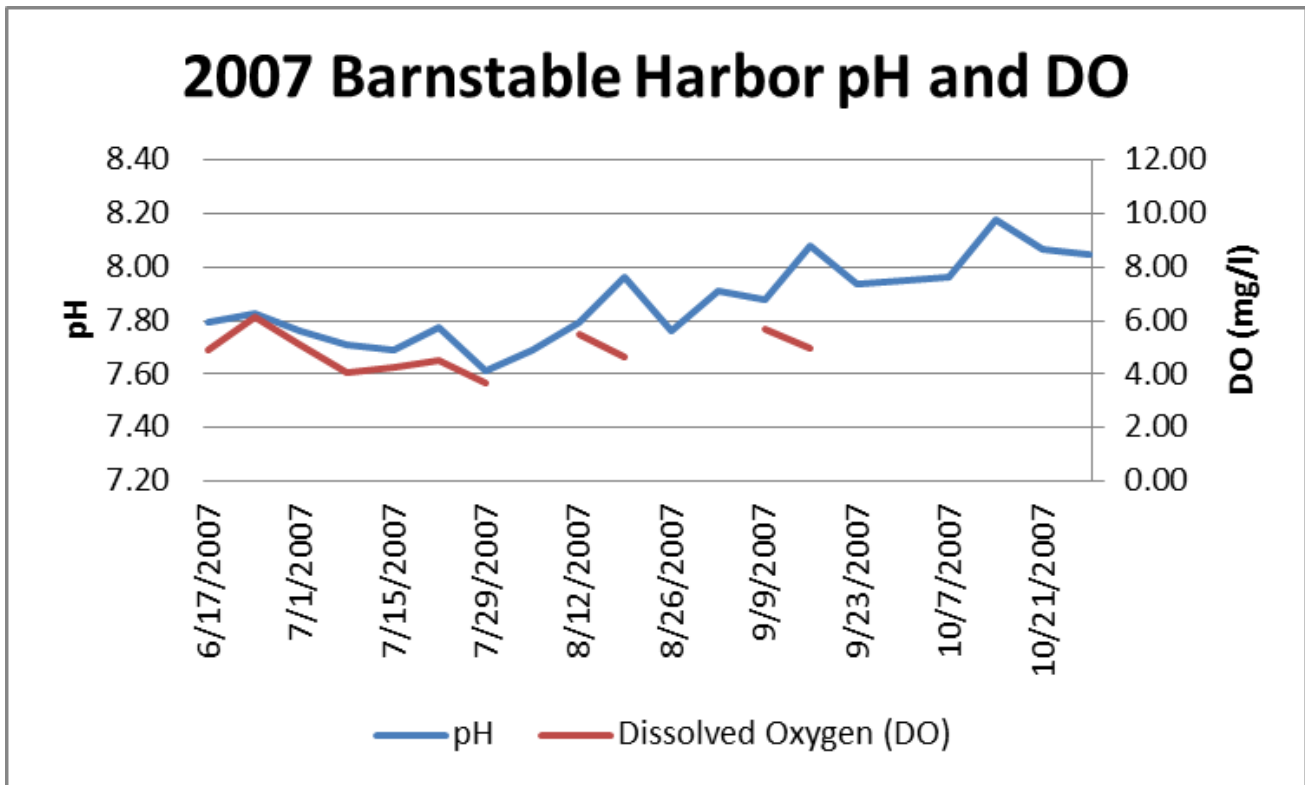
Weekly mean pH and dissolved oxygen as measured at the Inner Harbor of Barnstable Harbor during 2007.
