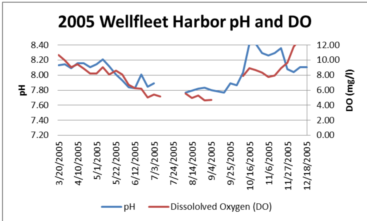
Weekly mean pH and dissolved oxygen as measured in Wellfleet Harbor during 2005.
