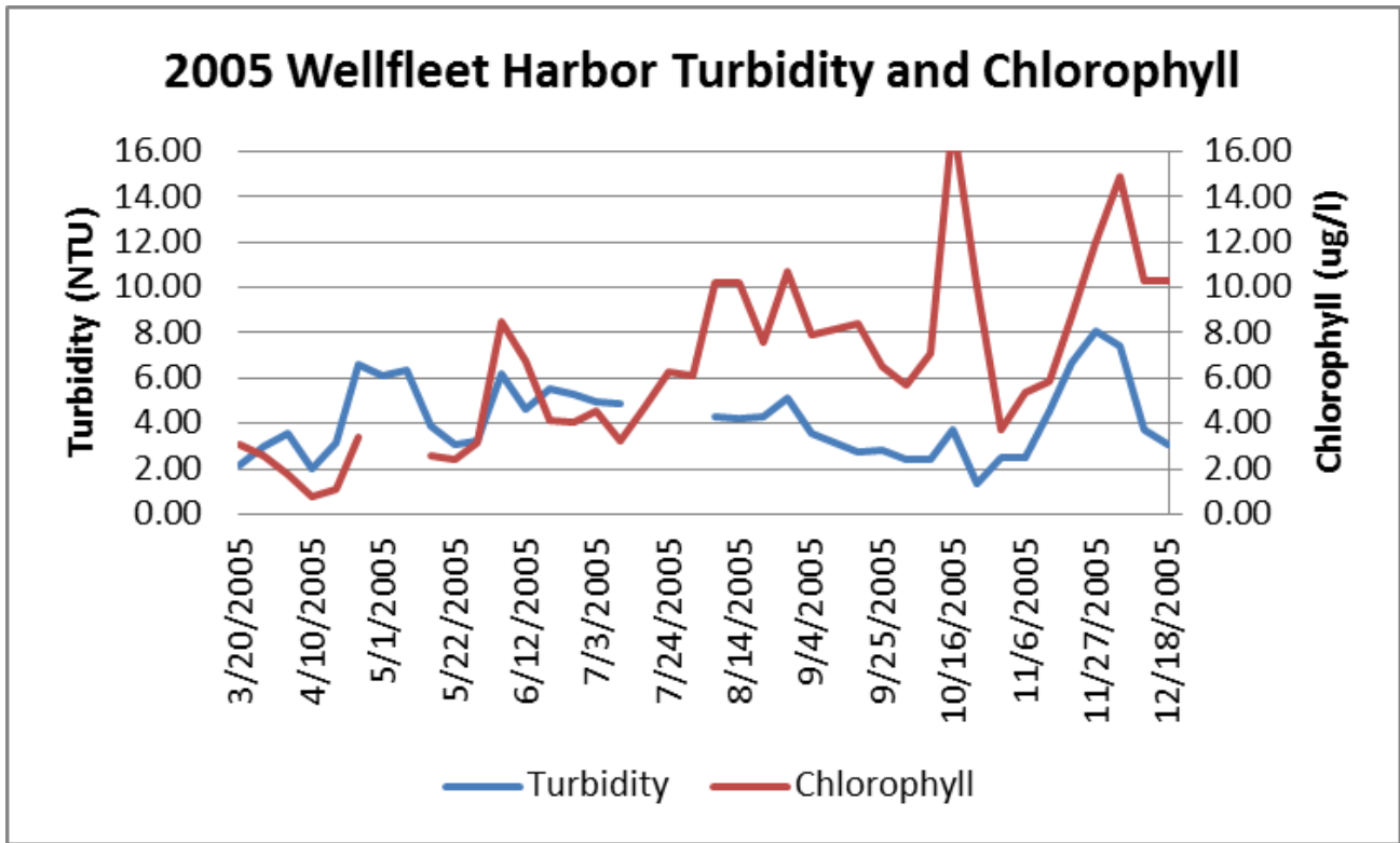
Weekly mean turbidity and chlorophyll as measured in Wellfleet Harbor during 2005.
