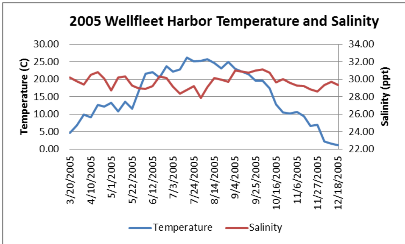
Weekly mean water temperature and salinity as measured in Wellfleet Harbor during 2005.
