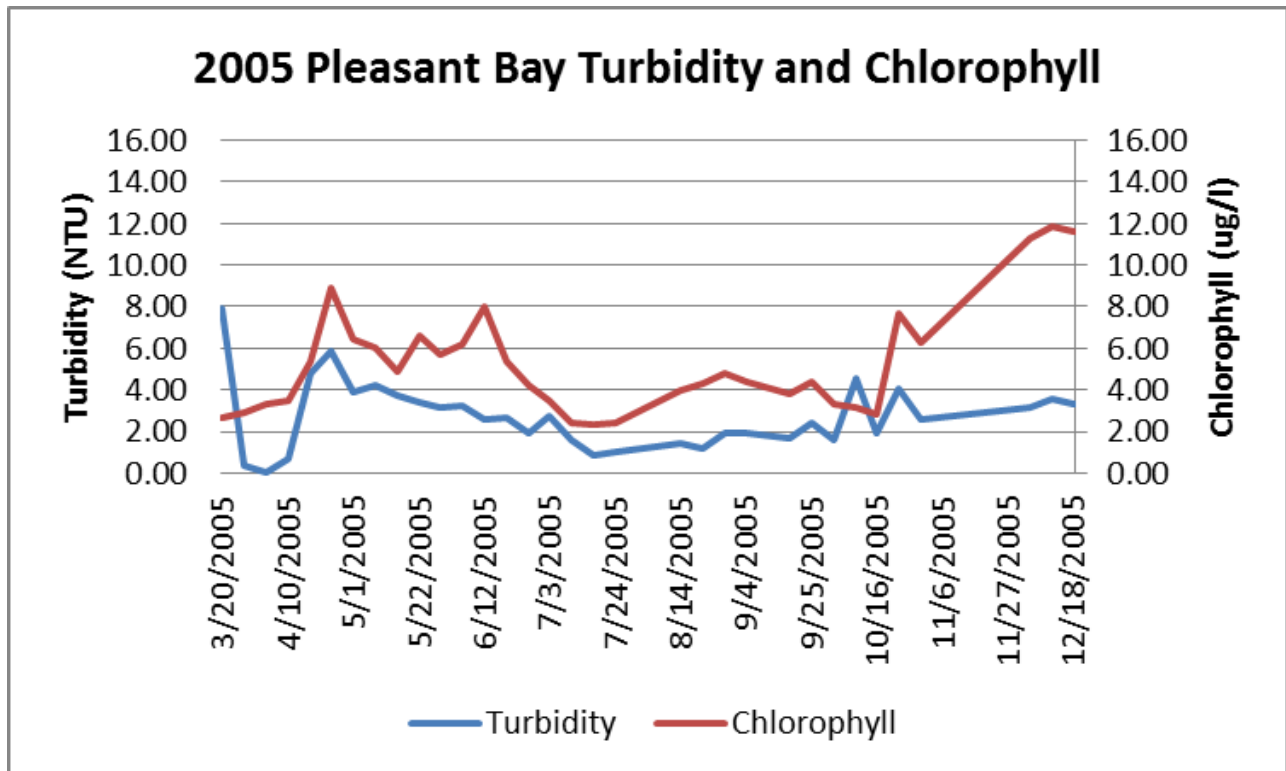
Weekly mean turbidity and chlorophyll as measured in Pleasant Bay at Portanimicut Landing during 2005.
