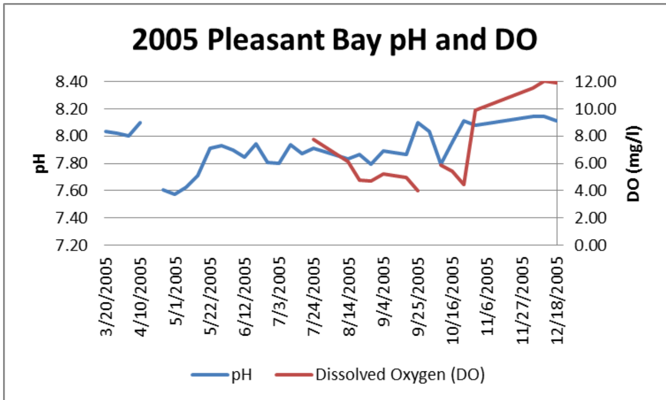
Weekly mean pH and dissolved oxygen as measured in Pleasant Bay at Portanimicut Landing during 2005.
