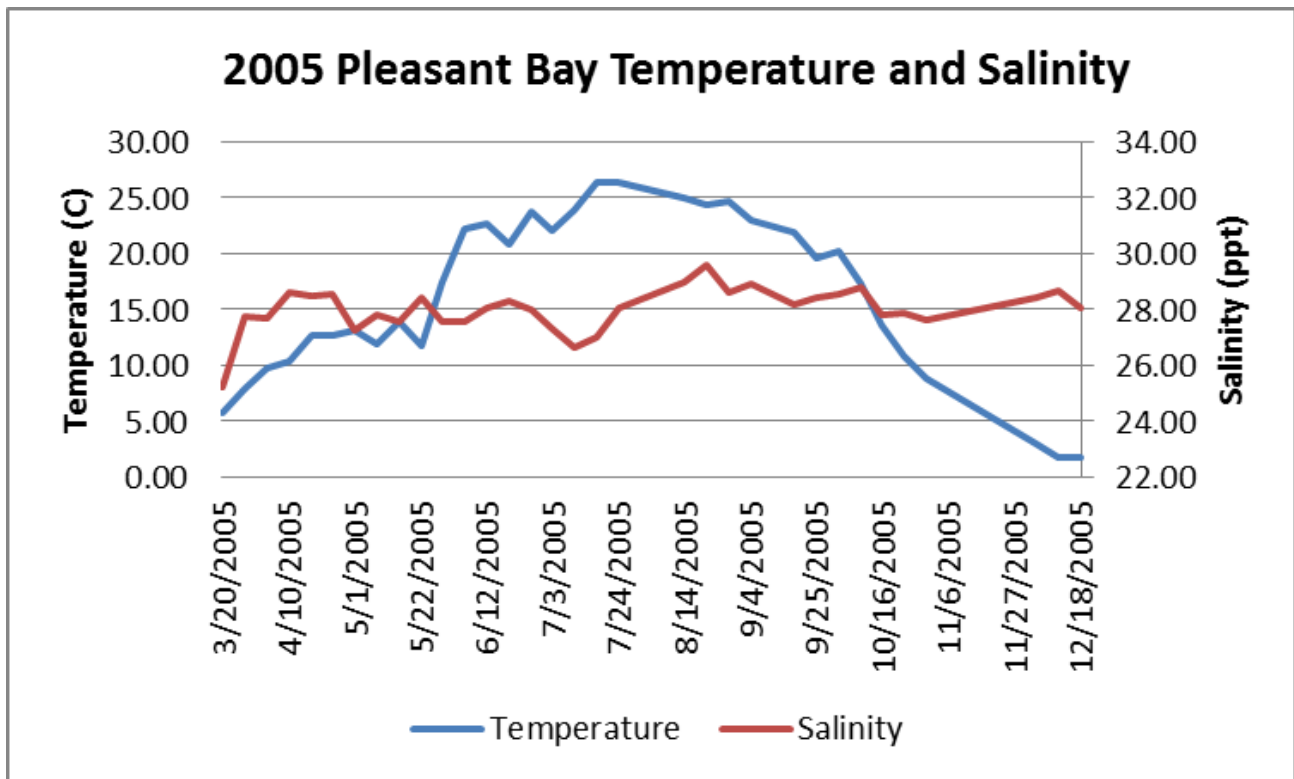
Weekly mean water temperature and salinity as measured in Pleasant Bay at Portanimicut Landing during 2005.
