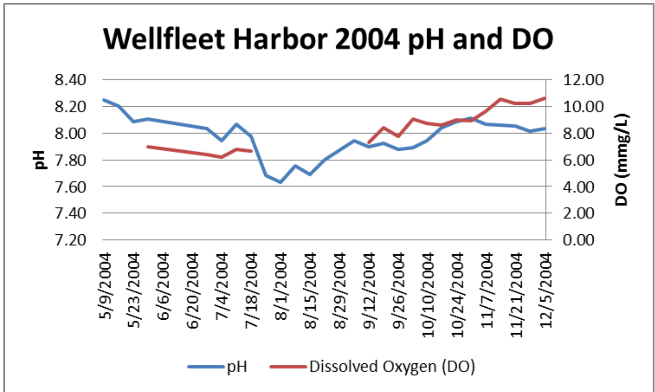
Weekly mean pH and dissolved oxygen as measured in Wellfleet Harbor during 2004.
