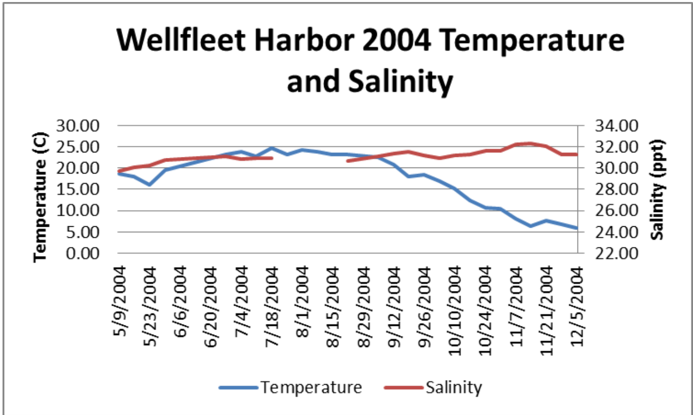
Weekly mean water temperature and salinity as measured in Wellfleet Harbor during 2004.
