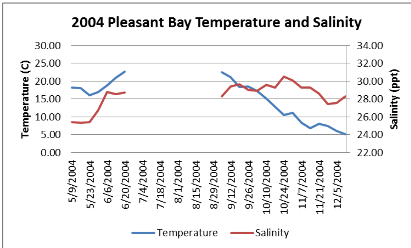
Weekly mean water temperature and salinity as measured in Pleasant Bay at Portanimicut Landing during 2004.
