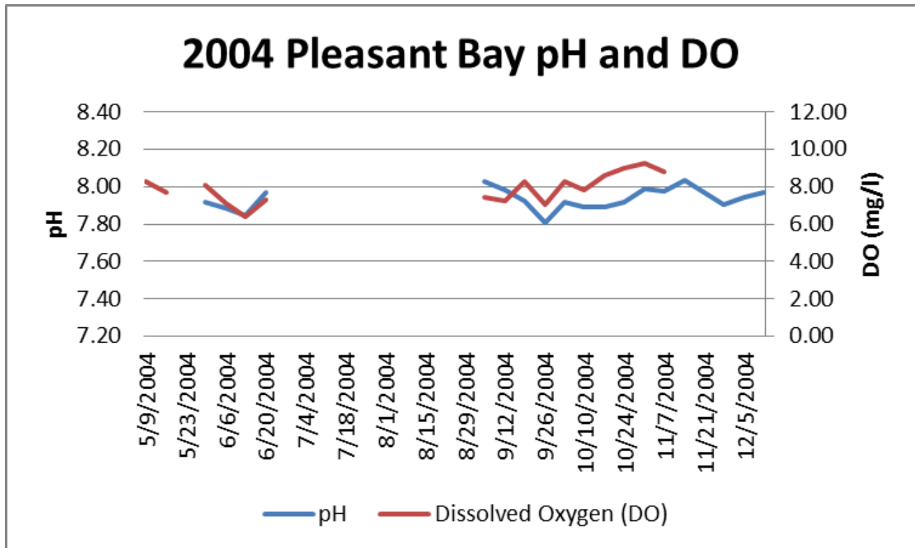
Weekly mean pH and dissolved oxygen as measured in Pleasant Bay at Portanimicut Landing during 2004.
