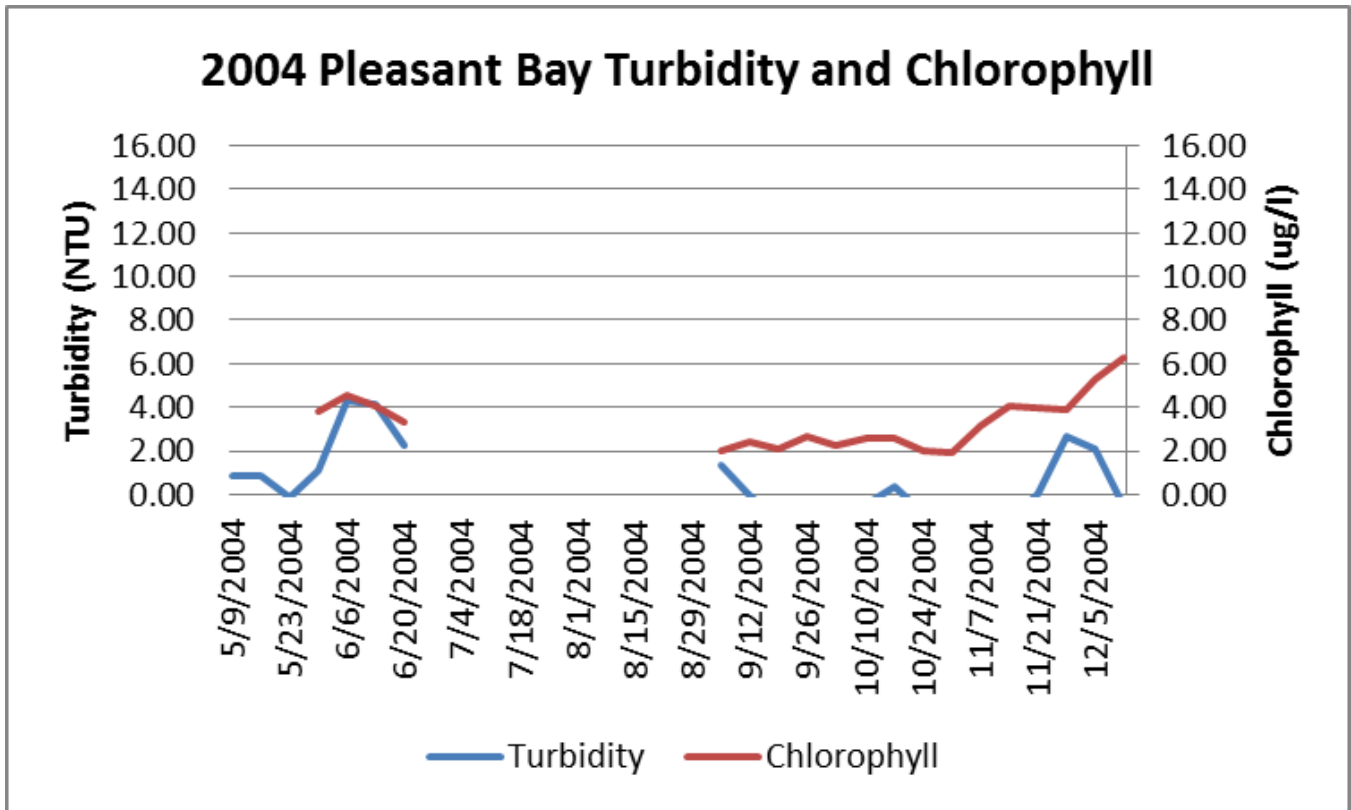
Weekly mean turbidity and chlorophyll as measured in Pleasant Bay at Portanimicut Landing during 2004.
